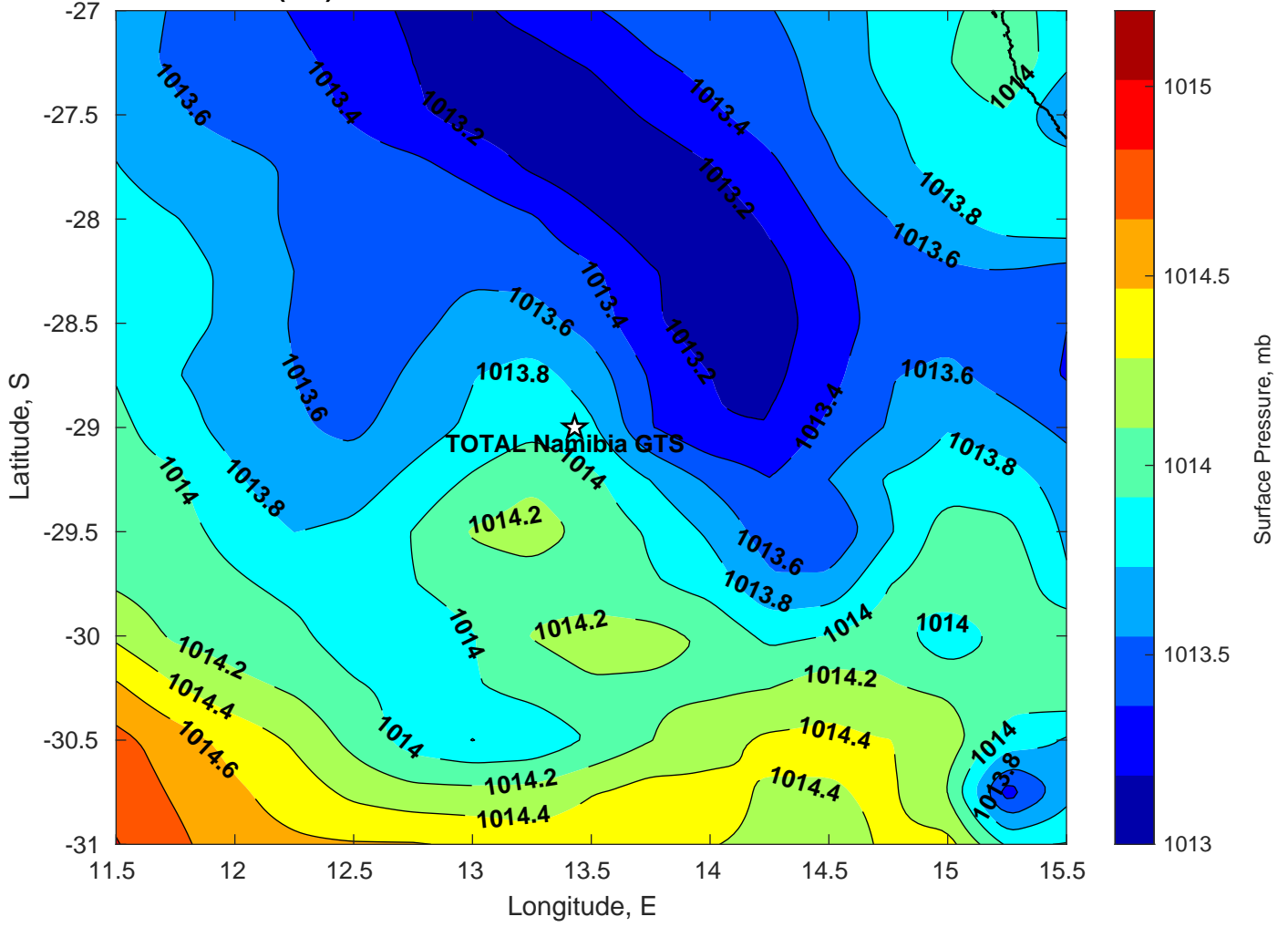
Surface Pressure (mb) for TOTAL Namibia GTS at 20-Mar-2025 12:00:00
