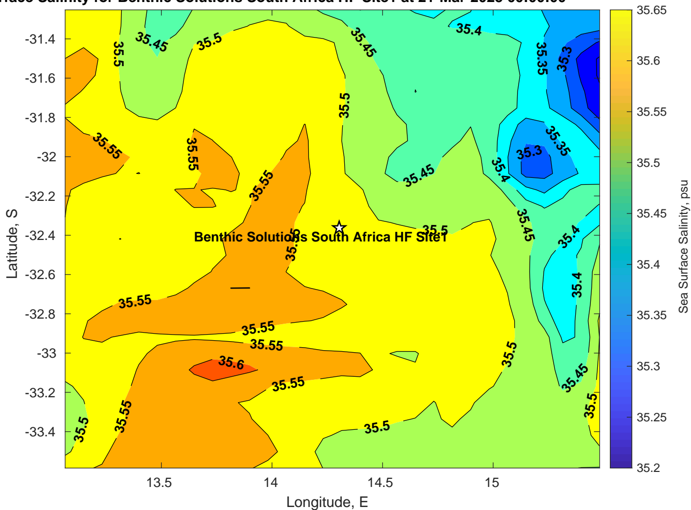
Surface Salinity for Benthic Solutions South Africa HF Site1 at 21-Mar-2025 00:00:00
