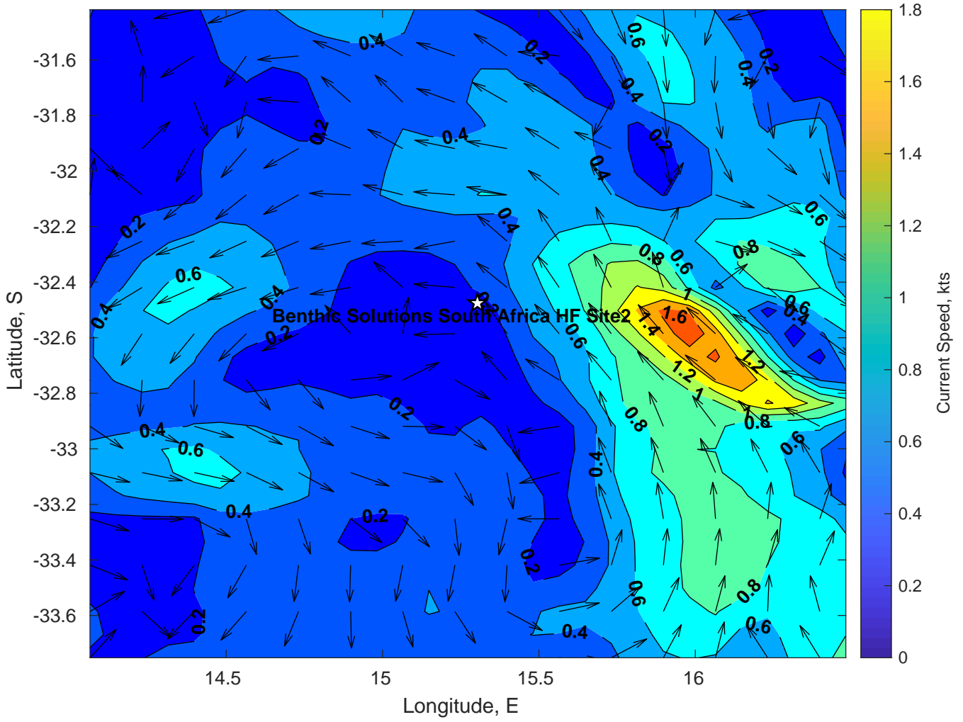
Surface Currents for Benthic Solutions South Africa HF Site2 at 21-Mar-2025 00:00:00
