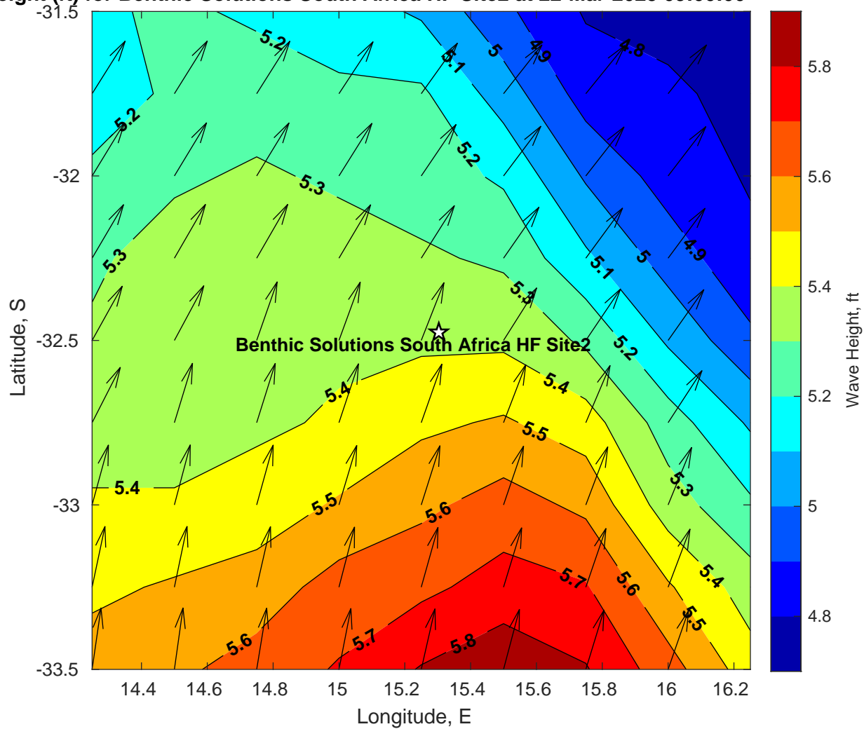
Wave Height (ft) for Benthic Solutions South Africa HF Site2 at 22-Mar-2025 09:00:00
