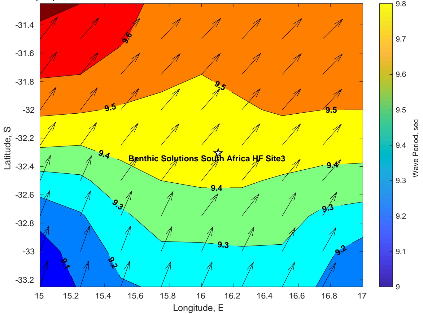
Wave Period (sec) for Benthic Solutions South Africa HF Site3 at 22-Mar-2025 09:00:00
