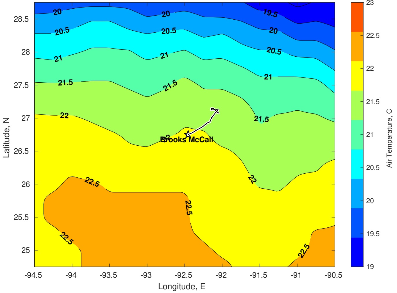
Air Temperature (C) for Brooks McCall at 22-Mar-2025
