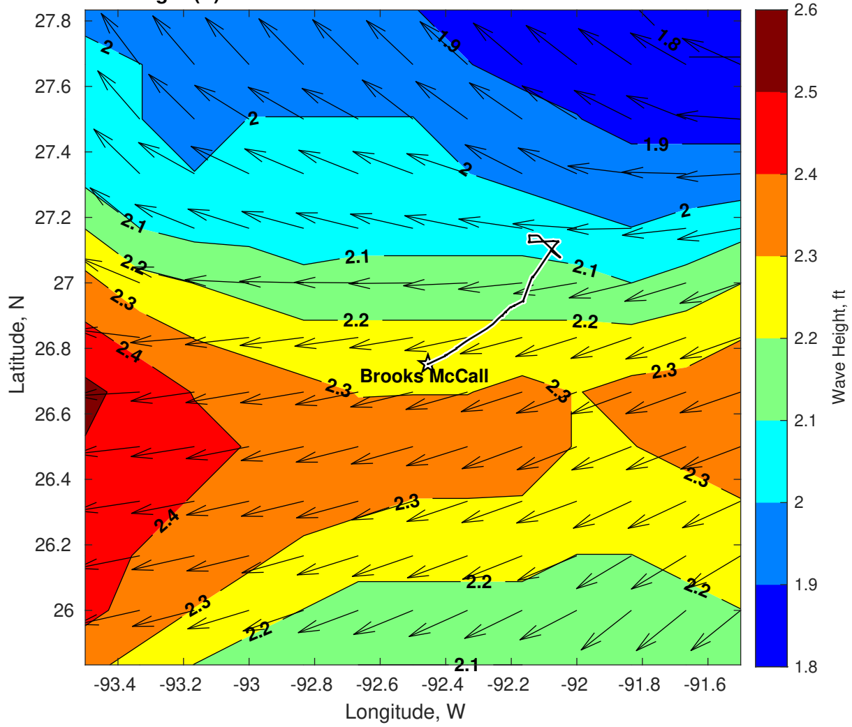
Wave Height (ft) for Brooks McCall at 22-Mar-2025 09:00:00
