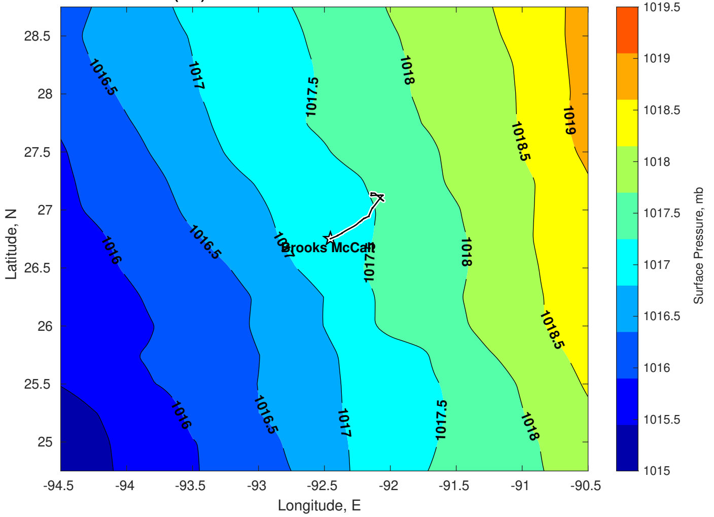
Surface Pressure (mb) for Brooks McCall at 23-Mar-2025 00:00:00
