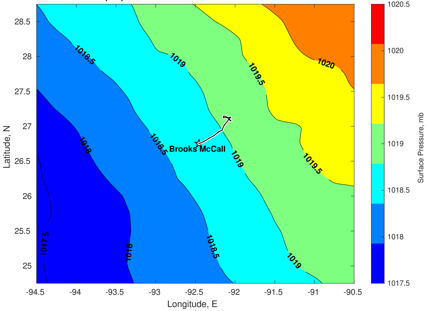
Surface Pressure (mb) for Brooks McCall at 22-Mar-2025 00:00:00
