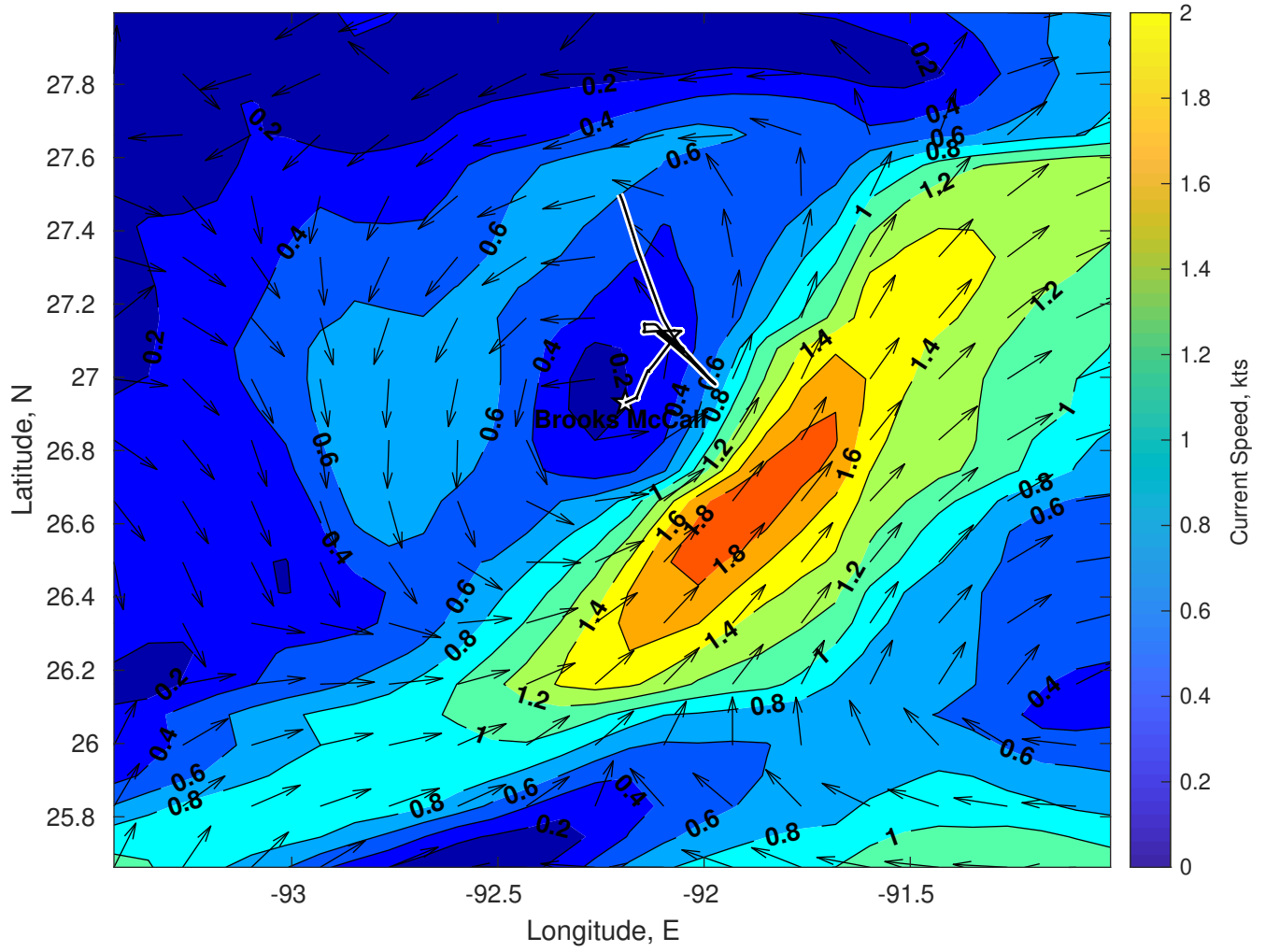
Surface Currents for Brooks McCall at 21-Mar-2025 00:00:00
