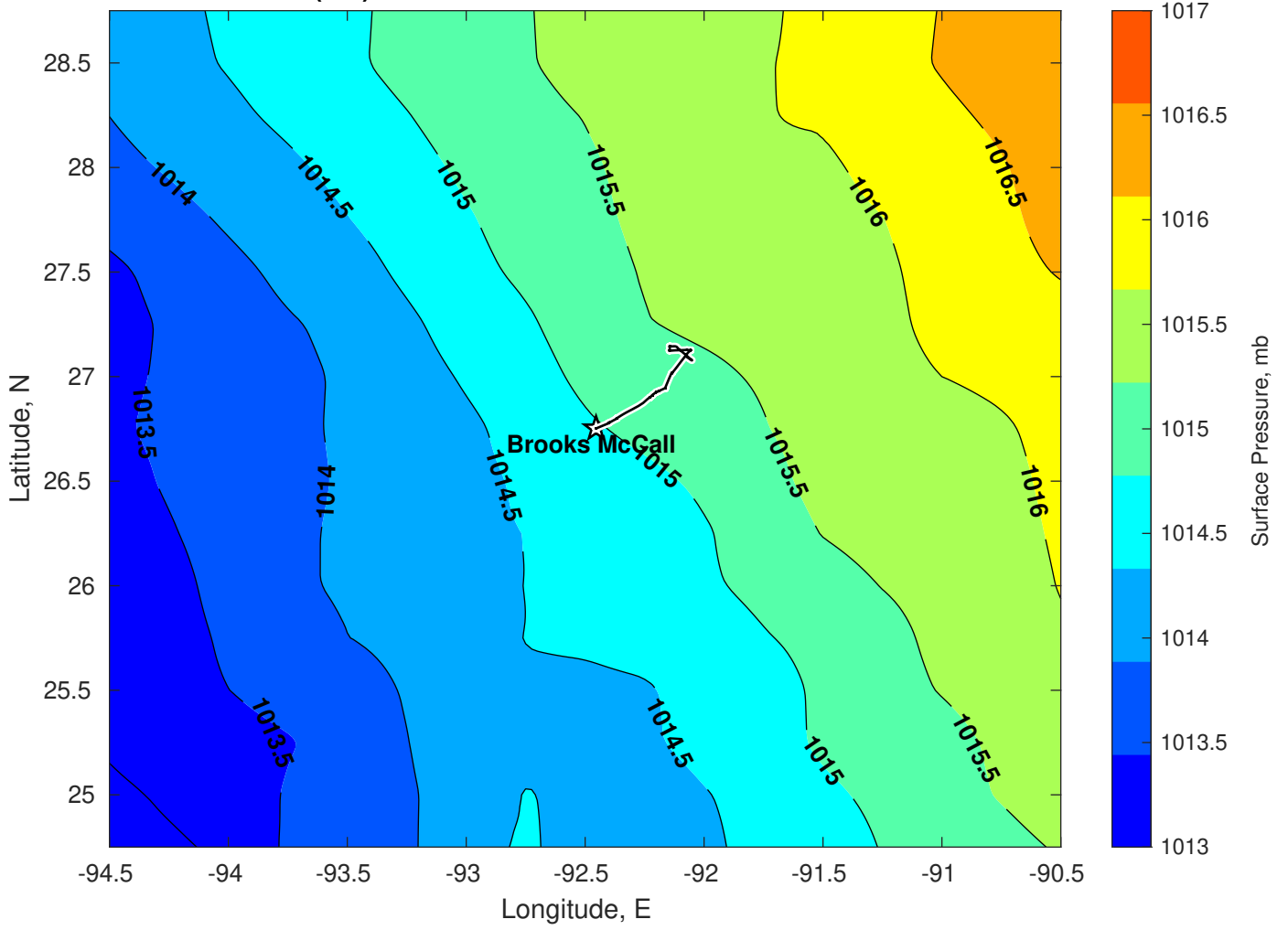
Surface Pressure (mb) for Brooks McCall at 24-Mar-2025 00:00:00
