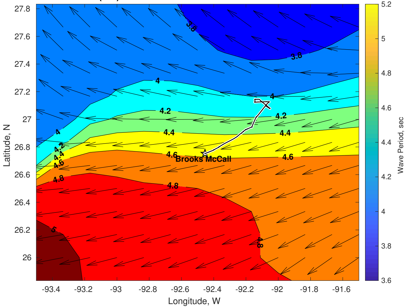
Wave Period (sec) for Brooks McCall at 22-Mar-2025 09:00:00
