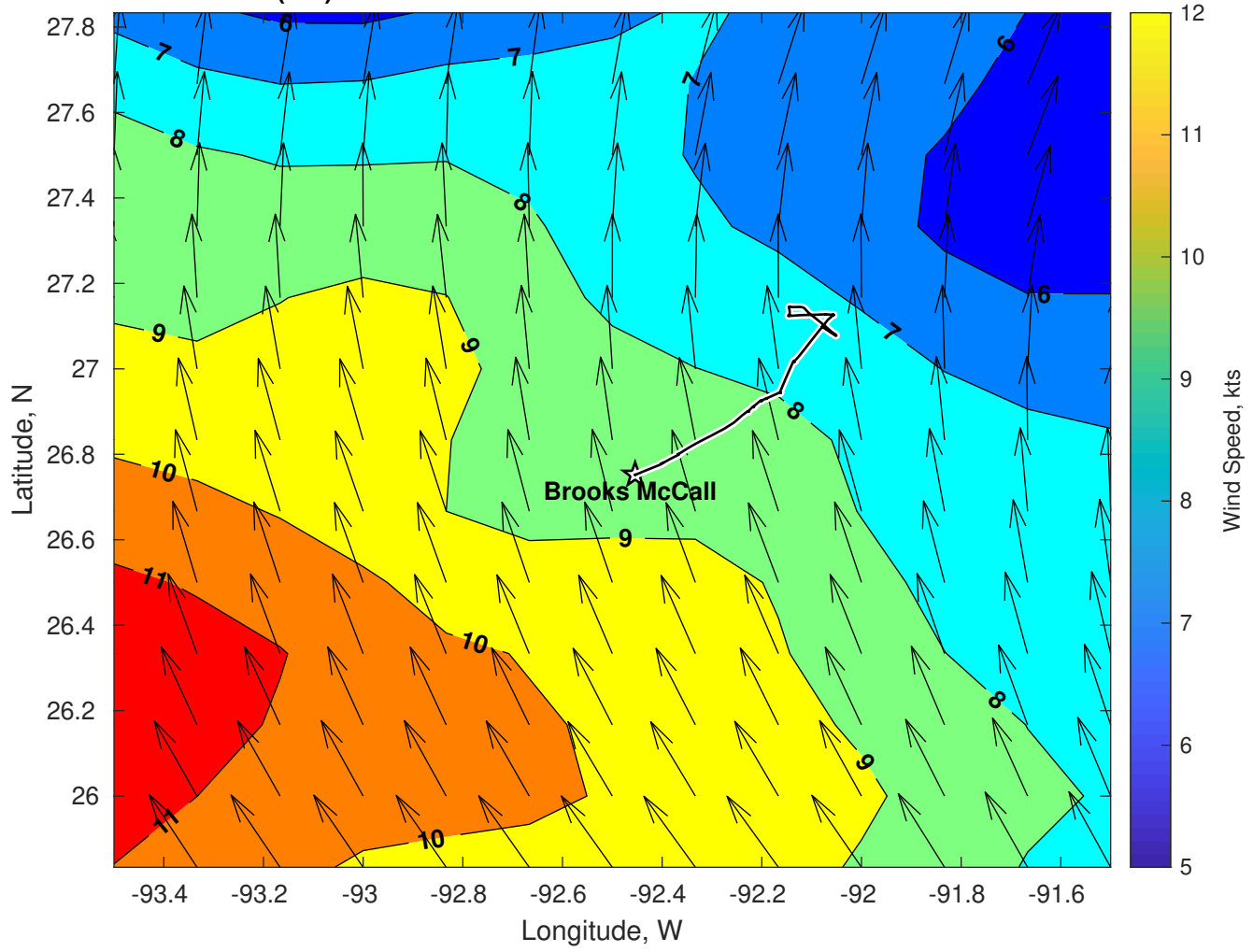
Winds (kts) for Brooks McCall at 22-Mar-2025 09:00:00
