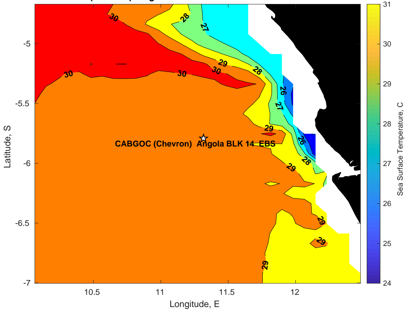
SST for CABGOC (Chevron) Angola BLK 14 EBS at 21-Mar-2025 00:00:00
