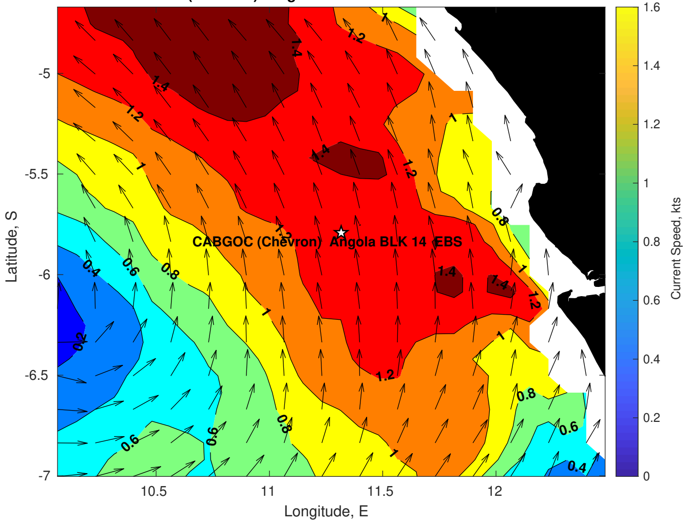
Surface Currents for CABGOC (Chevron) Angola BLK 14 EBS at 21-Mar-2025 00:00:00
