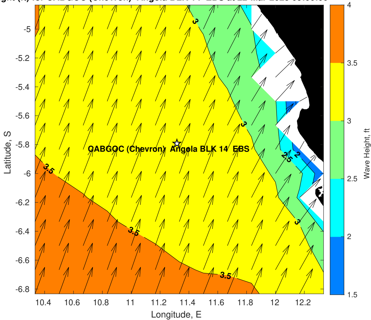
Wave Height (ft) for CABGOC (Chevron) Angola BLK 14 EBS at 22-Mar-2025 09:00:00
