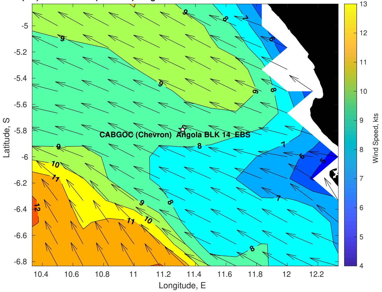
Winds (kts) for CABGOC (Chevron) Angola BLK 14 EBS at 22-Mar-2025 09:00:00
