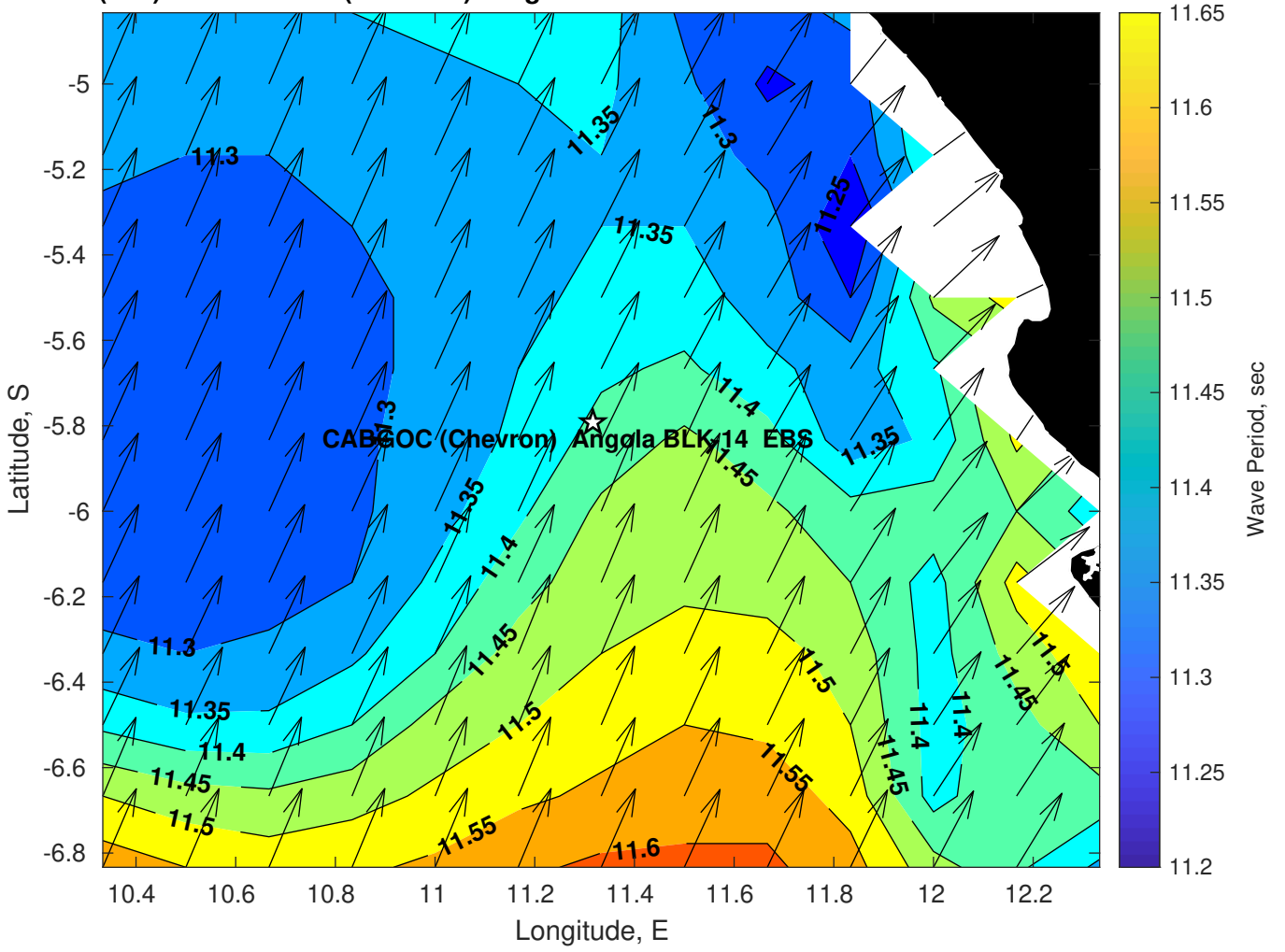
Wave Period (sec) for CABGOC (Chevron) Angola BLK 14 EBS at 22-Mar-2025 09:00:00
