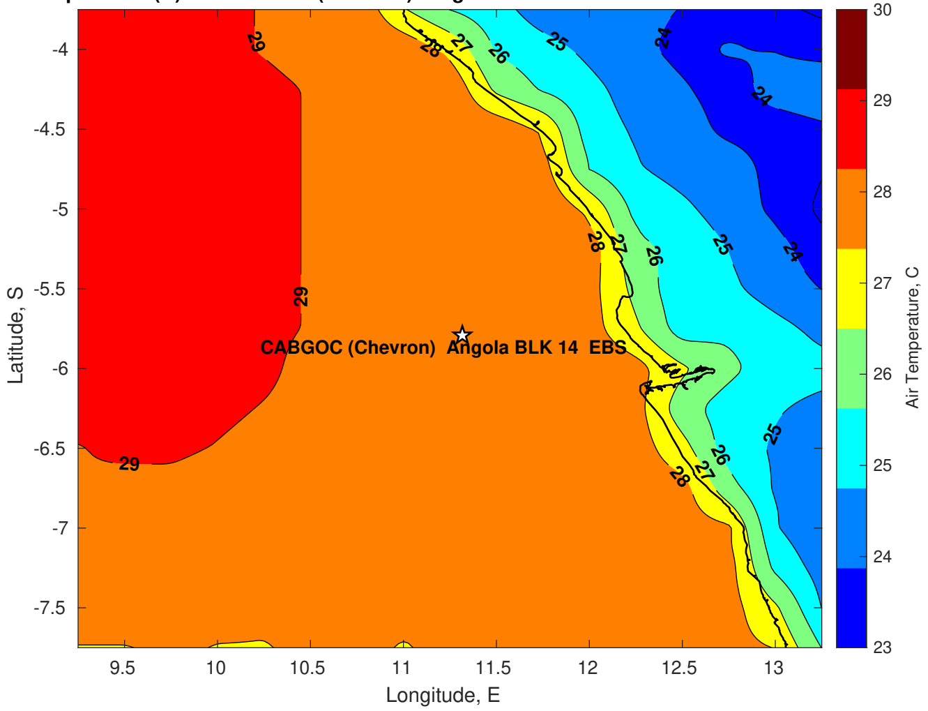
Air Temperature (C) for CABGOC (Chevron) Angola BLK 14 EBS at 22-Mar-2025
