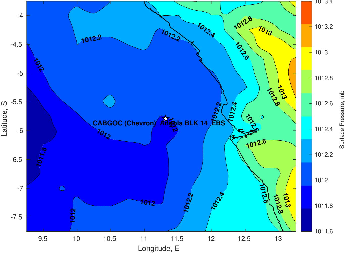
Surface Pressure (mb) for CABGOC (Chevron) Angola BLK 14 EBS at 22-Mar-2025 00:00:00
