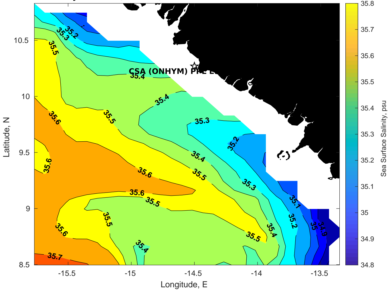
Surface Salinity for CSA (ONHYM) PPL EBS - Guinea at 21-Mar-2025 00:00:00
