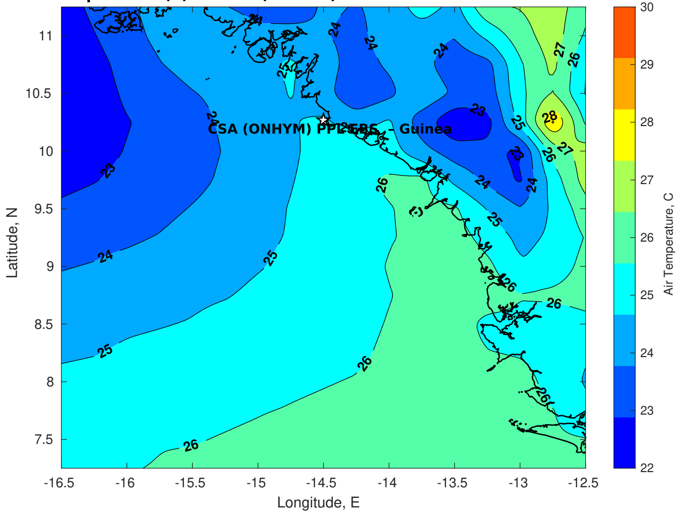
Air Temperature (C) for CSA (ONHYM) PPL EBS - Guinea at 22-Mar-2025
