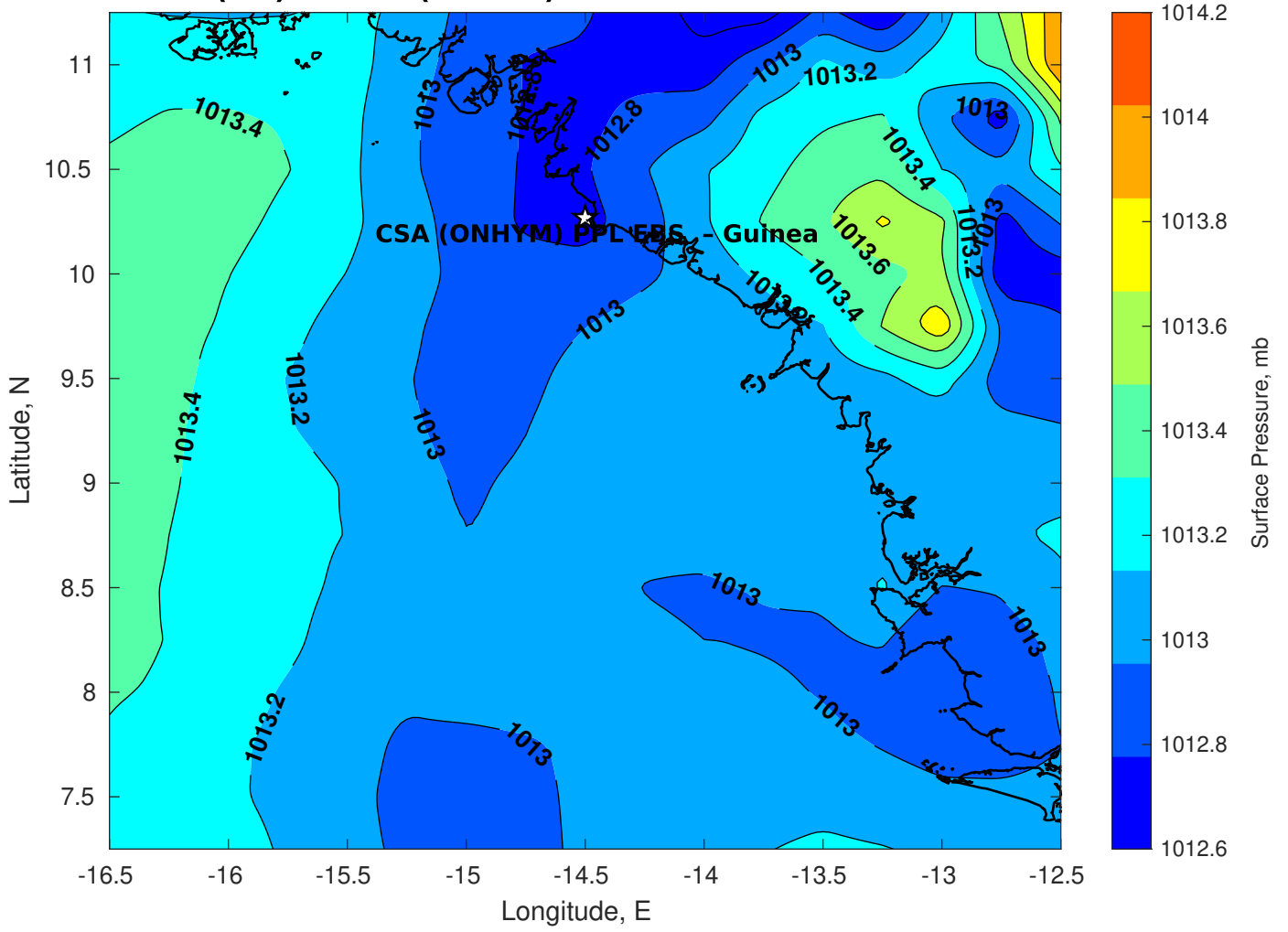
Surface Pressure (mb) for CSA (ONHYM) PPL EBS - Guinea at 24-Mar-2025 00:00:00
