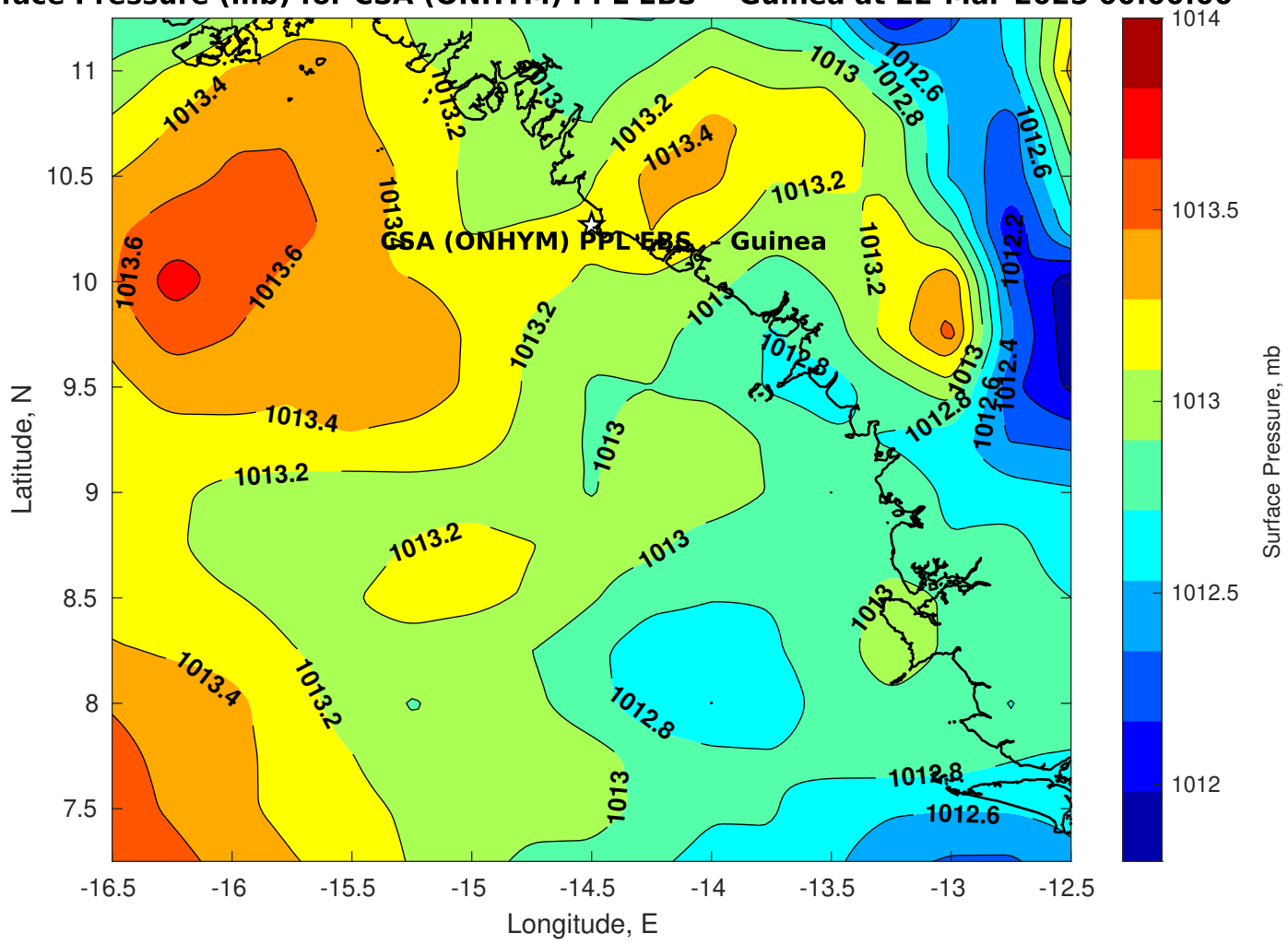
Surface Pressure (mb) for CSA (ONHYM) PPL EBS - Guinea at 22-Mar-2025 00:00:00
