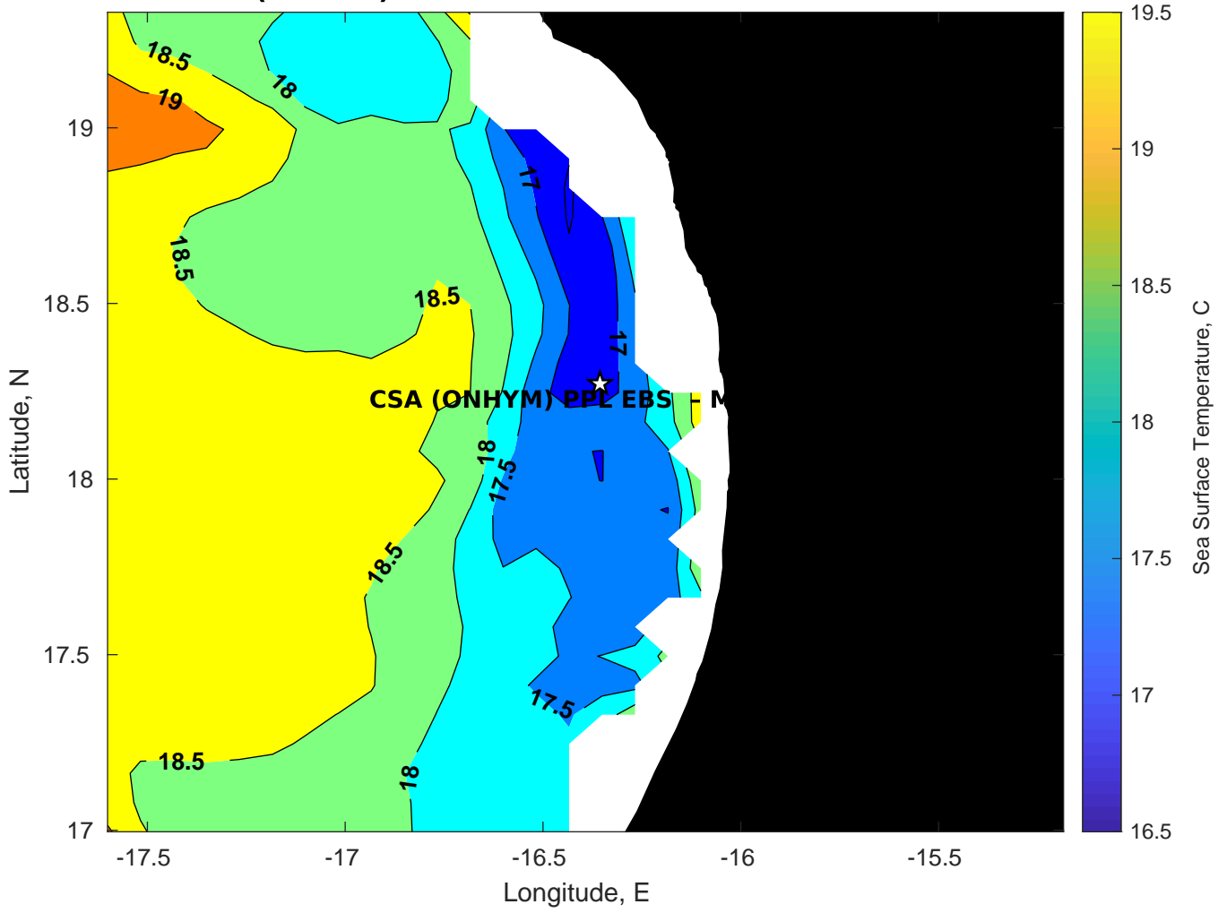
SST for CSA (ONHYM) PPL EBS - Mauritania at 21-Mar-2025 00:00:00
