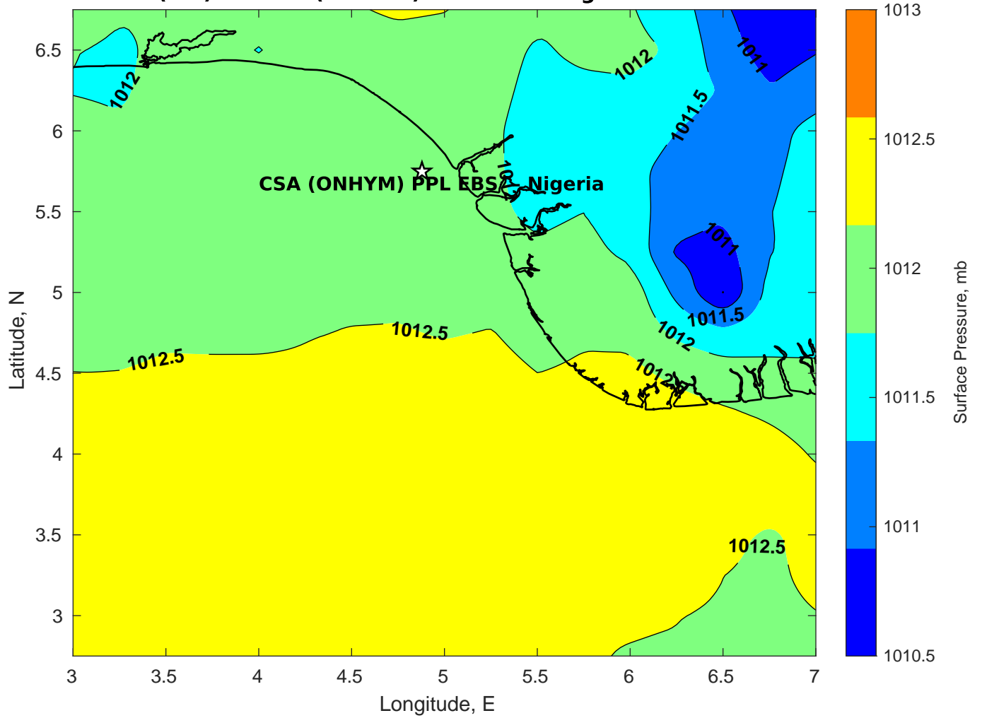
Surface Pressure (mb) for CSA (ONHYM) PPL EBS - Nigeria at 22-Mar-2025 00:00:00
