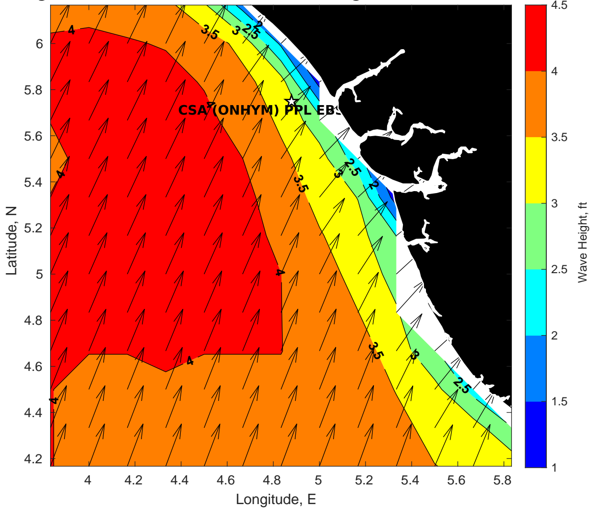
Wave Height (ft) for CSA (ONHYM) PPL EBS - Nigeria at 22-Mar-2025 09:00:00
