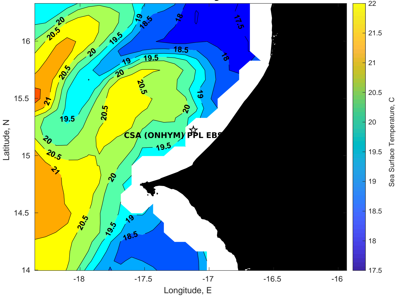
SST for CSA (ONHYM) PPL EBS - Senegal at 21-Mar-2025 00:00:00
