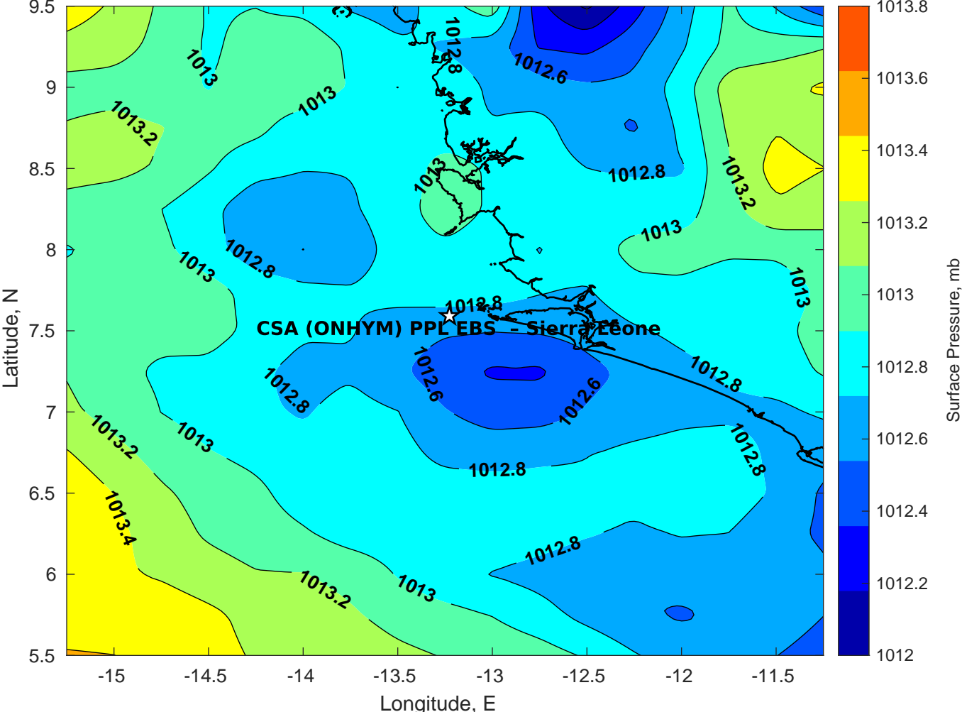
Surface Pressure (mb) for CSA (ONHYM) PPL EBS - Sierra Leone at 22-Mar-2025 00:00:00
