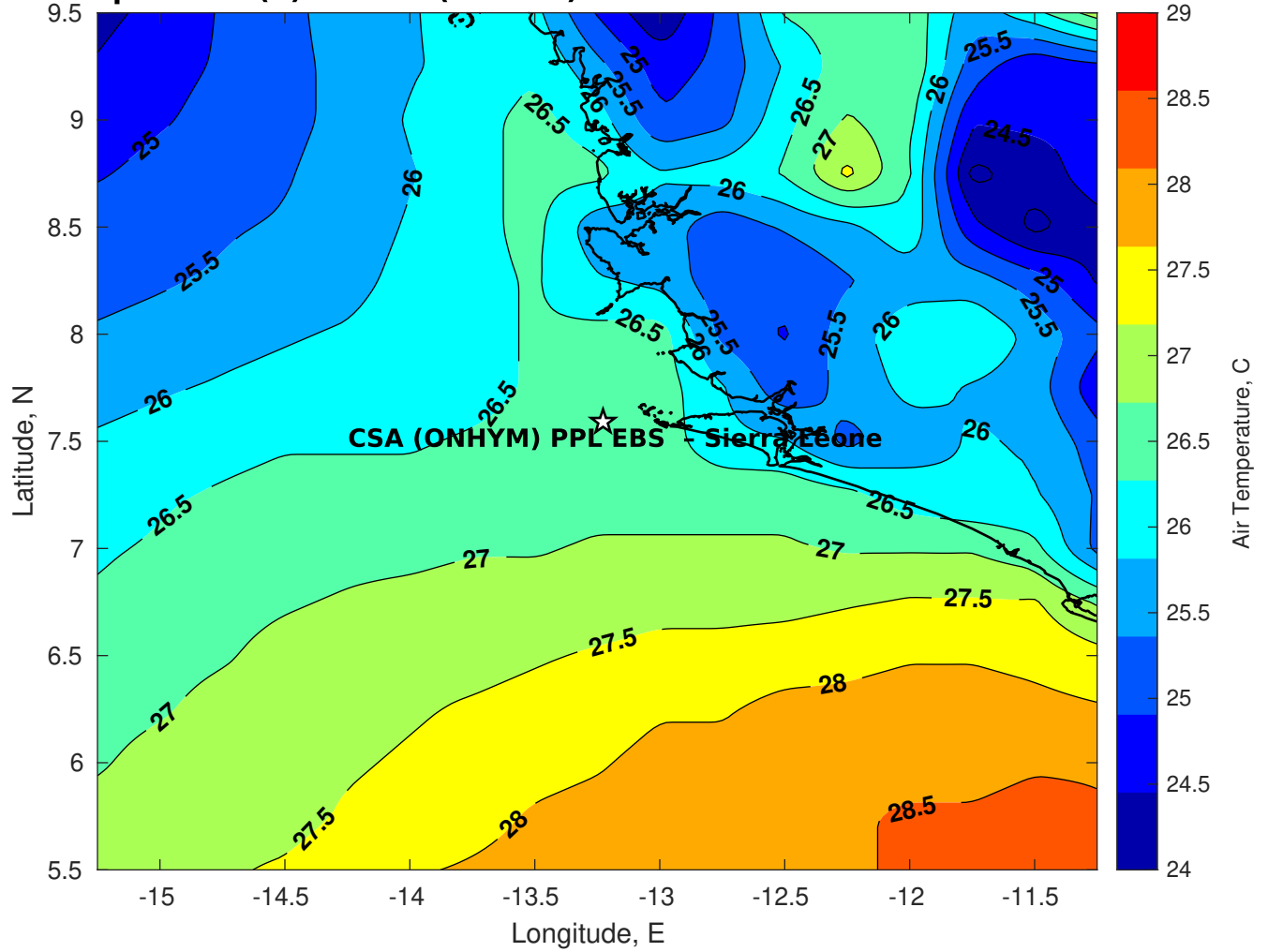
Air Temperature (C) for CSA (ONHYM) PPL EBS - Sierra Leone at 22-Mar-2025
