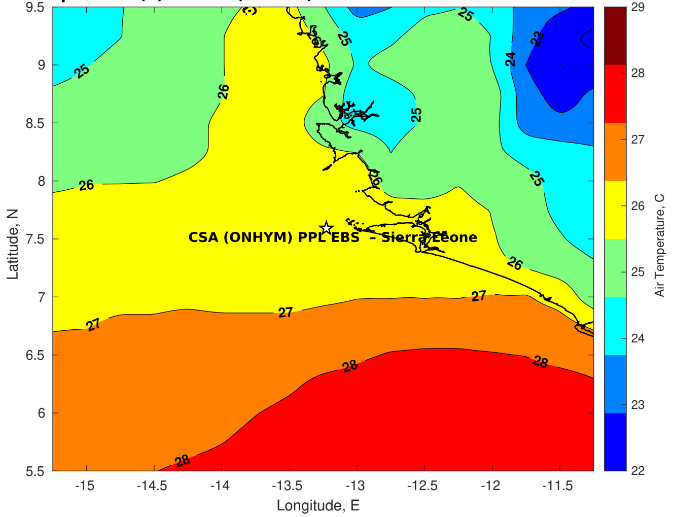
Air Temperature (C) for CSA (ONHYM) PPL EBS - Sierra Leone at 22-Mar-2025
