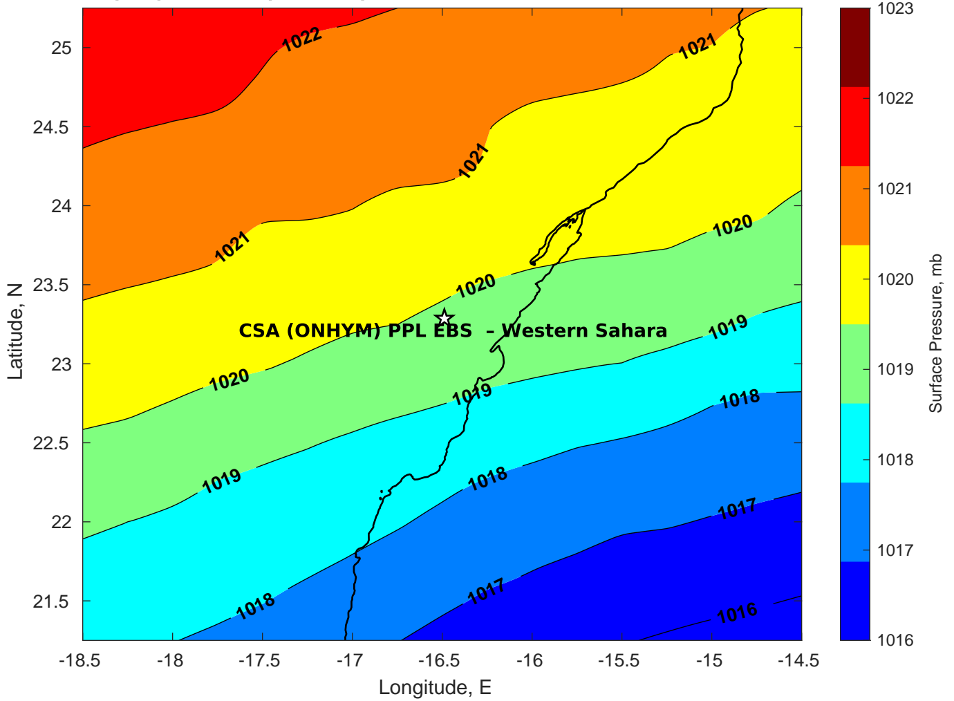
Surface Pressure (mb) for CSA (ONHYM) PPL EBS - Western Sahara at 24-Mar-2025 00:00:00
