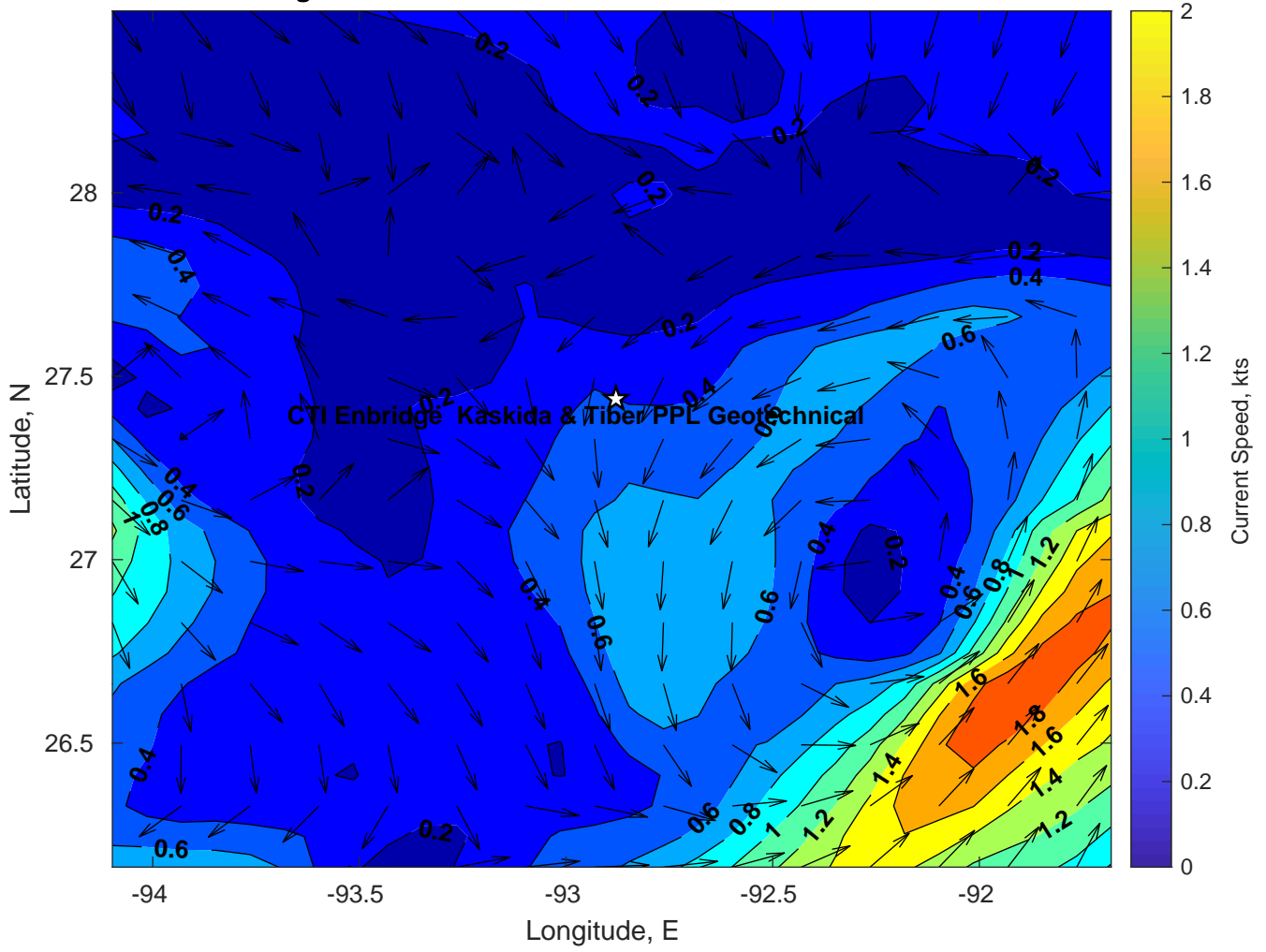
Surface Currents for CTI Enbridge Kaskida & Tiber PPL Geotechnical at 21-Mar-2025 00:00:00
