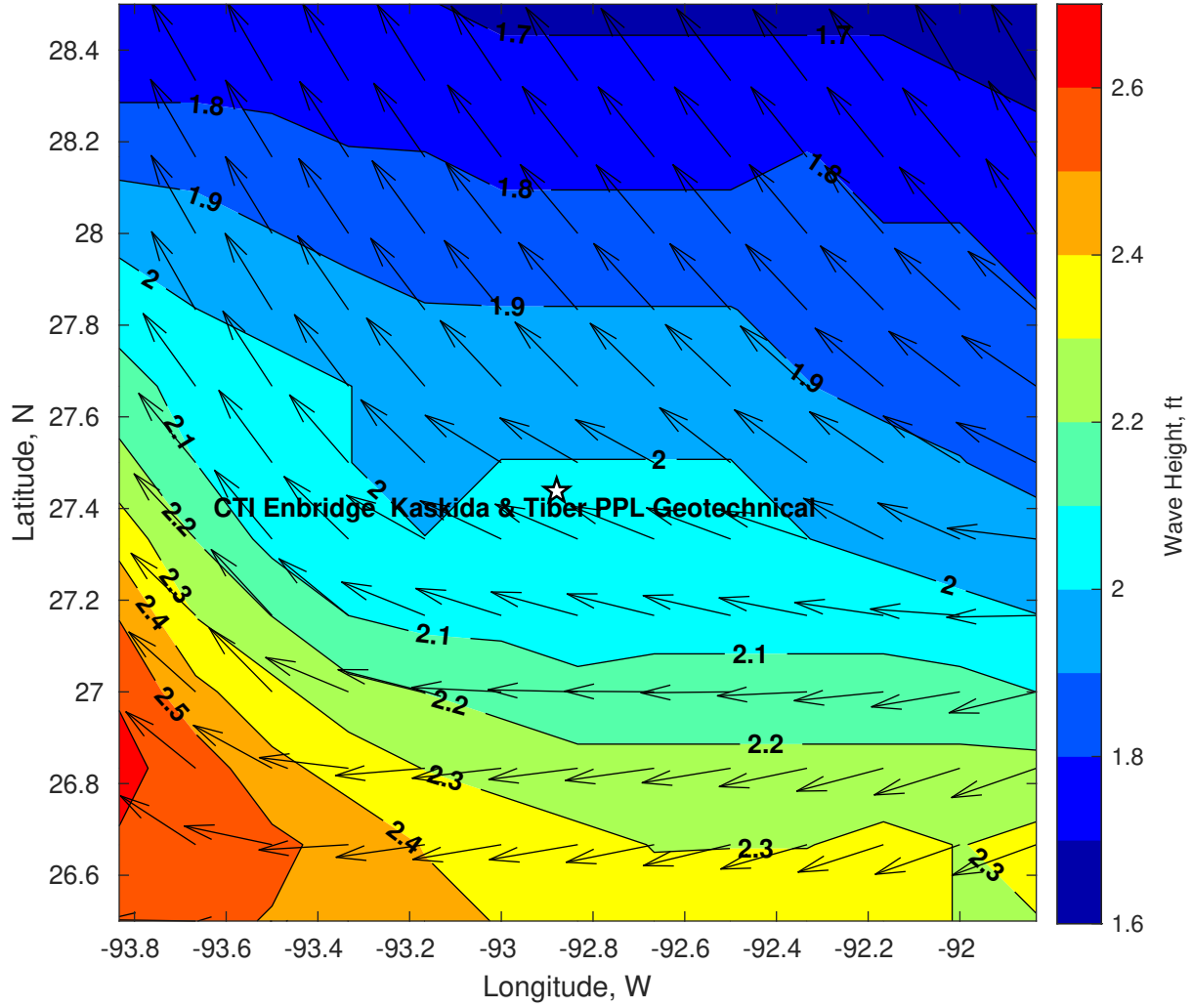
Wave Height (ft) for CTI Enbridge Kaskida & Tiber PPL Geotechnical at 22-Mar-2025 09:00:00
