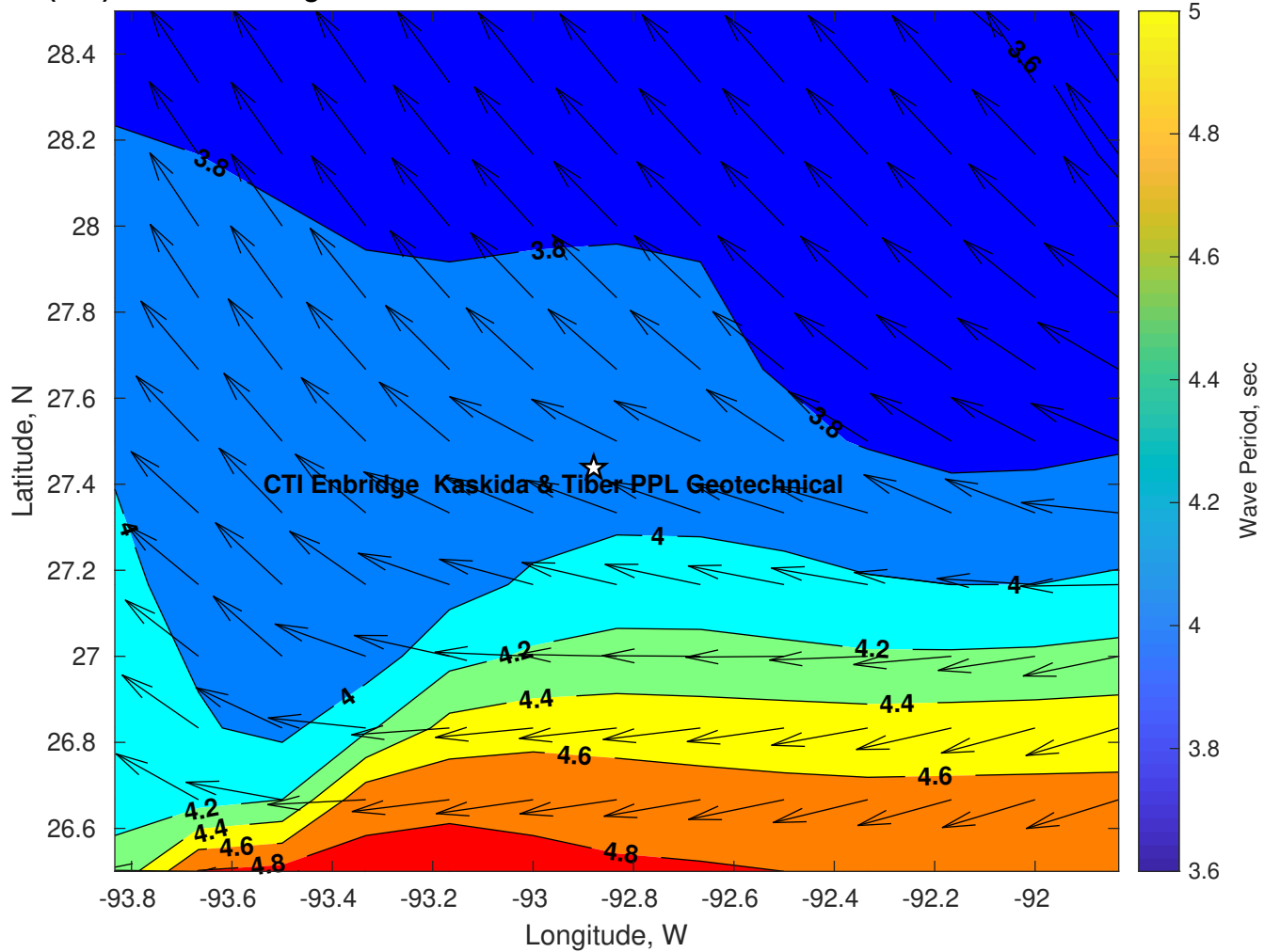
Wave Period (sec) for CTI Enbridge Kaskida & Tiber PPL Geotechnical at 22-Mar-2025 09:00:00
