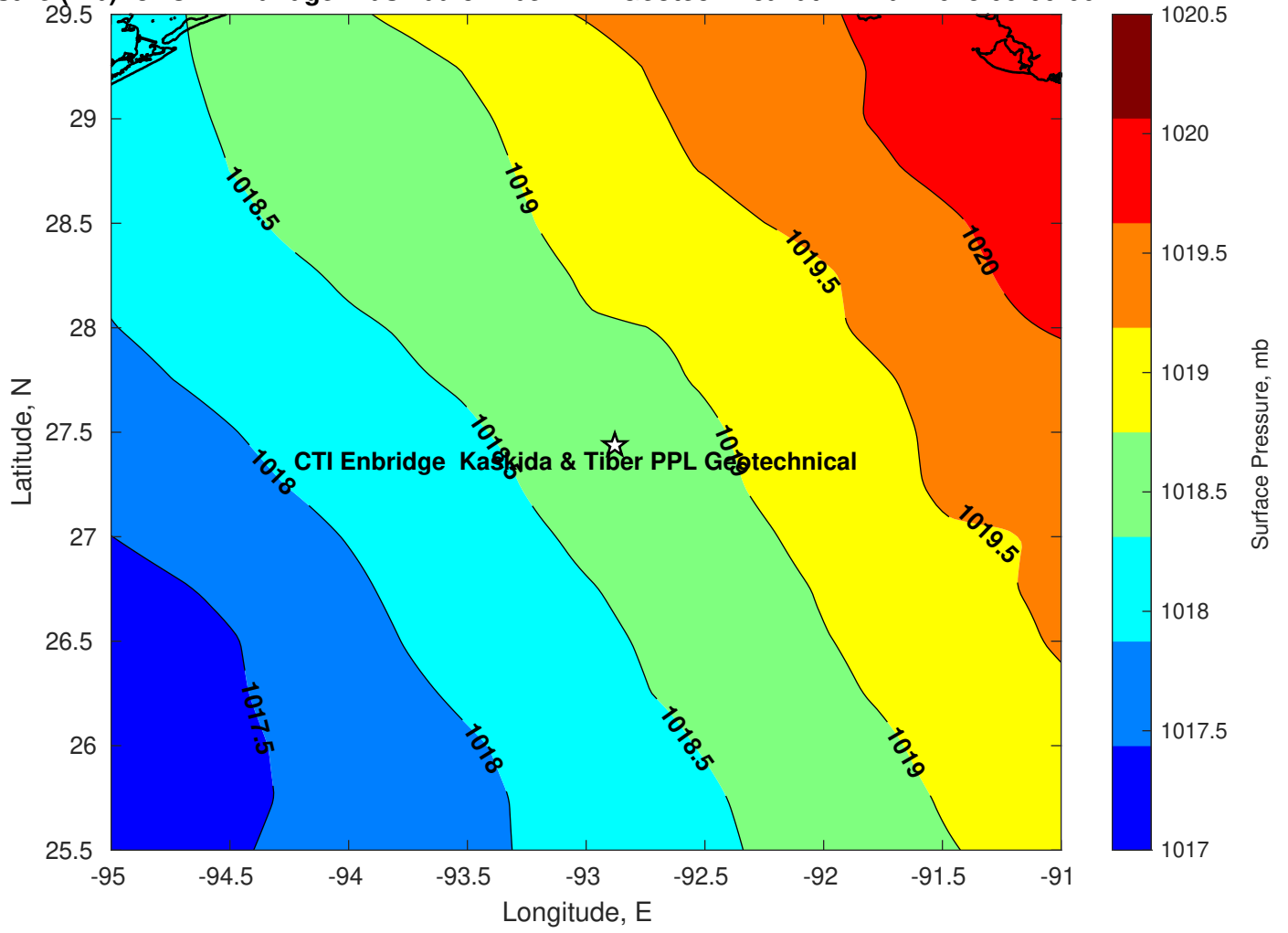
Surface Pressure (mb) for CTI Enbridge Kaskida & Tiber PPL Geotechnical at 22-Mar-2025 00:00:00
