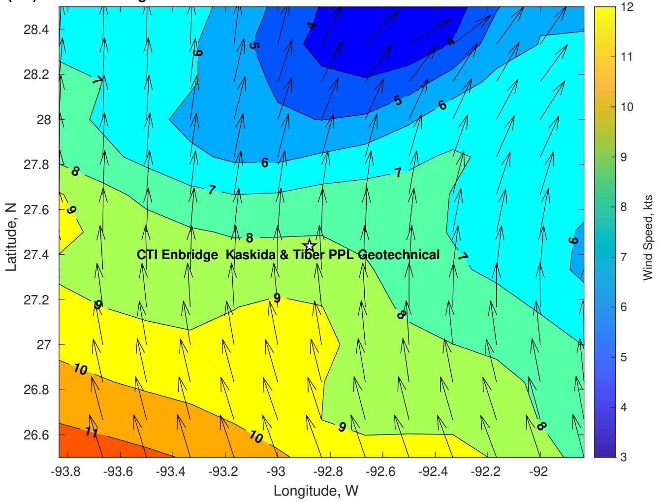
Winds (kts) for CTI Enbridge Kaskida & Tiber PPL Geotechnical at 22-Mar-2025 09:00:00
