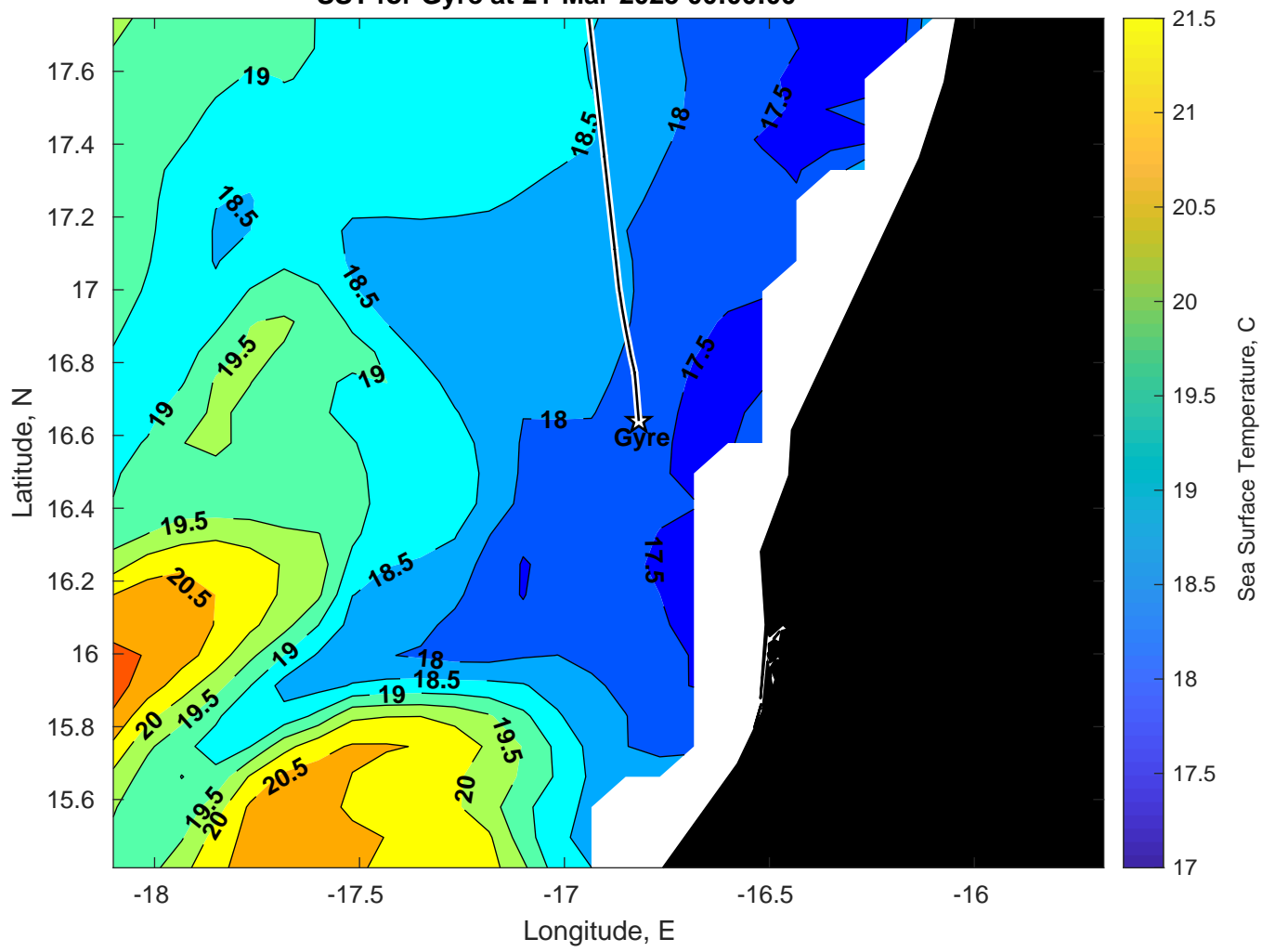
SST for Gyre at 21-Mar-2025 00:00:00
