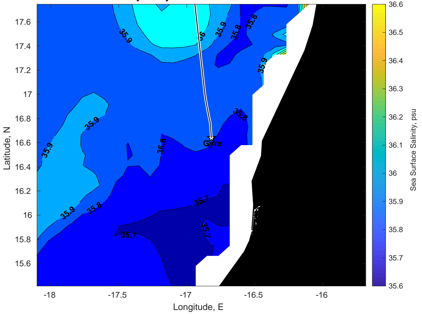
Surface Salinity for Gyre at 21-Mar-2025 00:00:00
