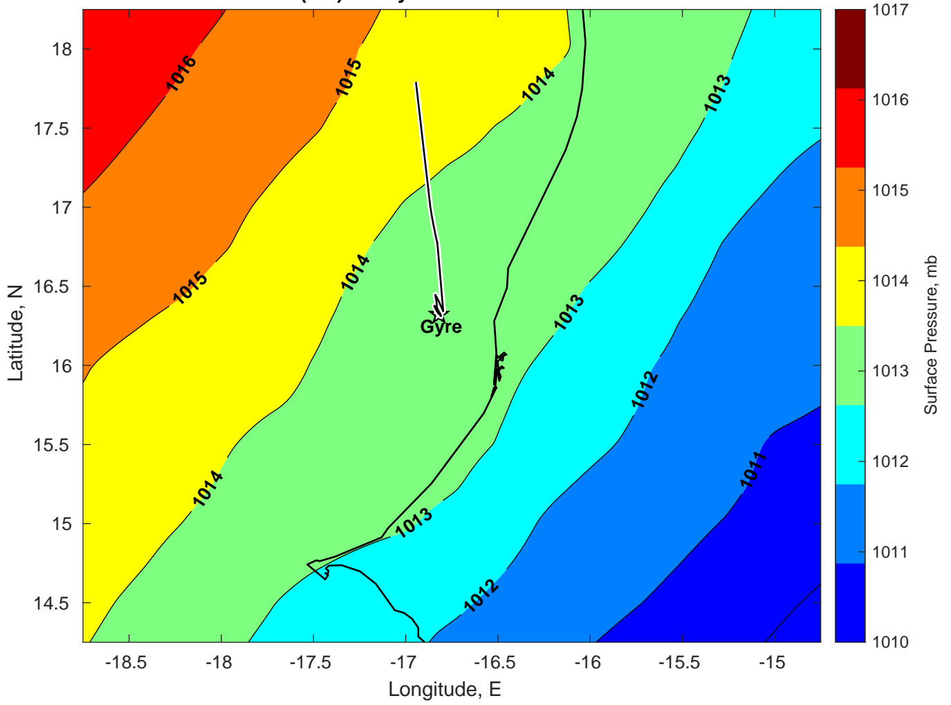
Surface Pressure (mb) for Gyre at 22-Mar-2025 00:00:00
