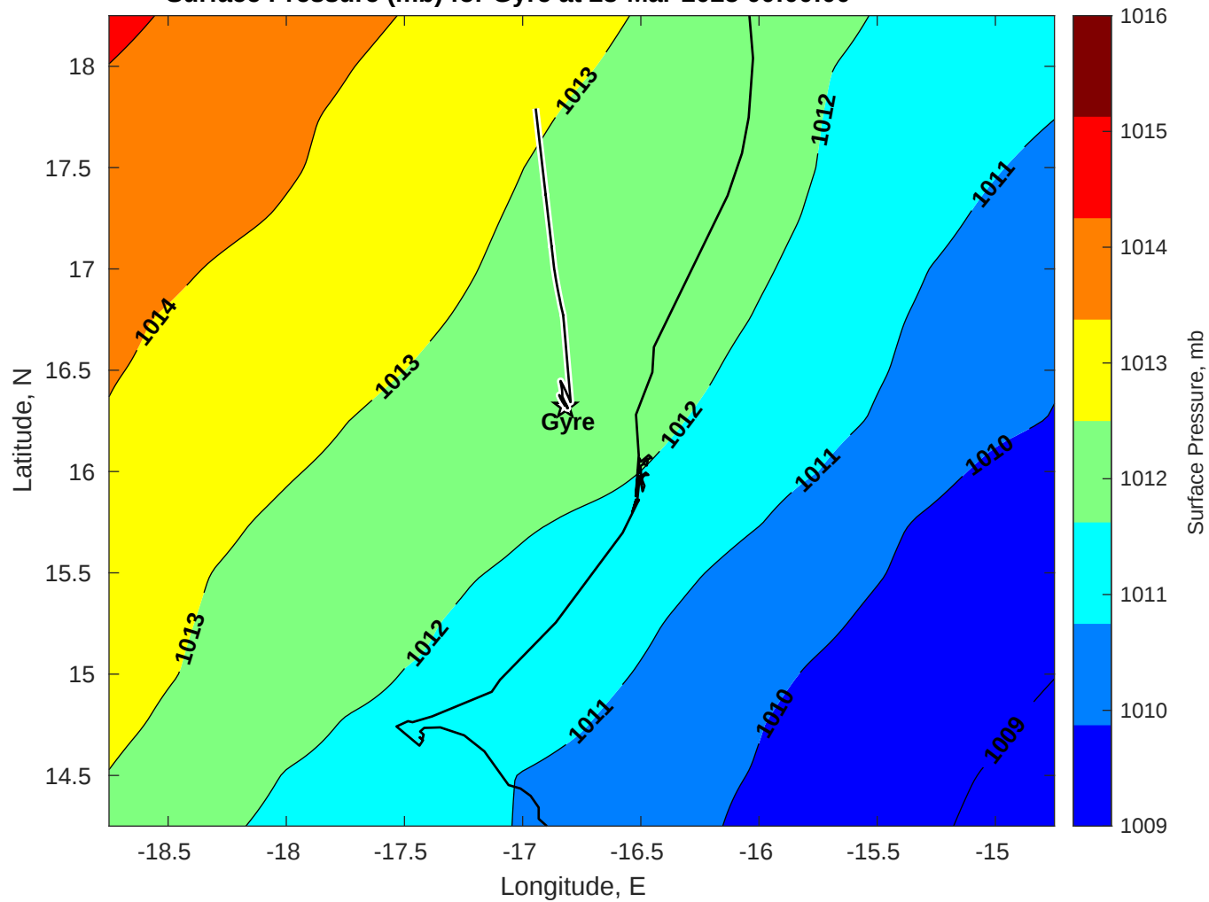
Surface Pressure (mb) for Gyre at 23-Mar-2025 00:00:00
