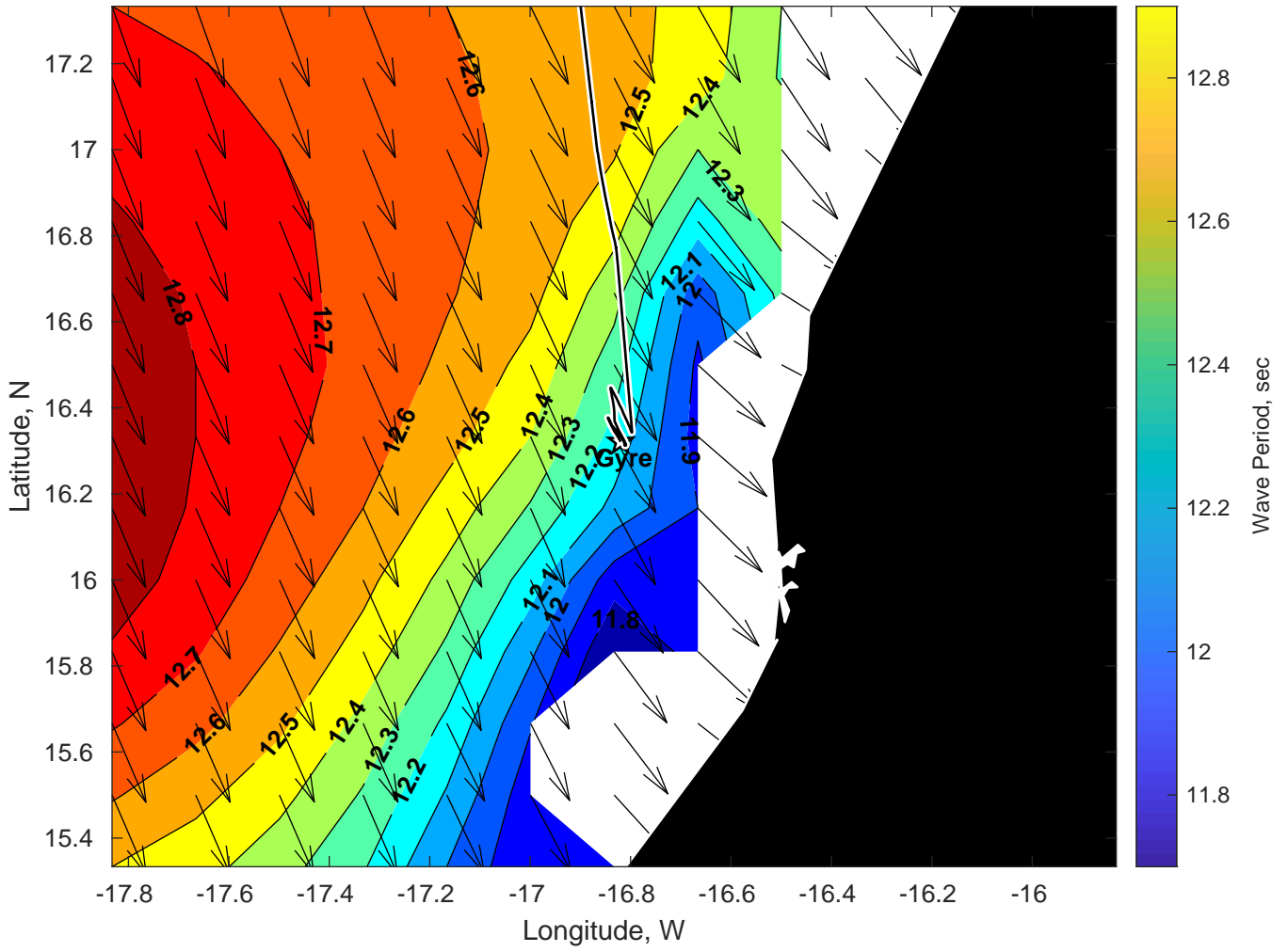
Wave Period (sec) for Gyre at 22-Mar-2025 09:00:00
