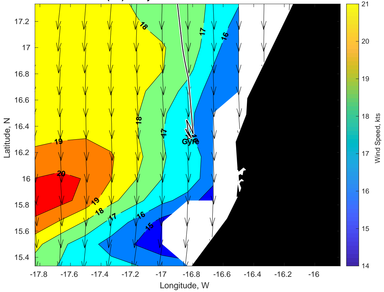
Winds (kts) for Gyre at 22-Mar-2025 09:00:00
