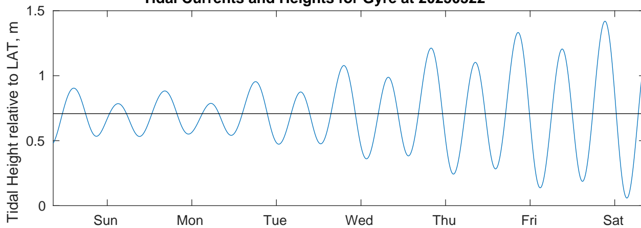
Tidal Currents and Heights for Gyre at 20250322
