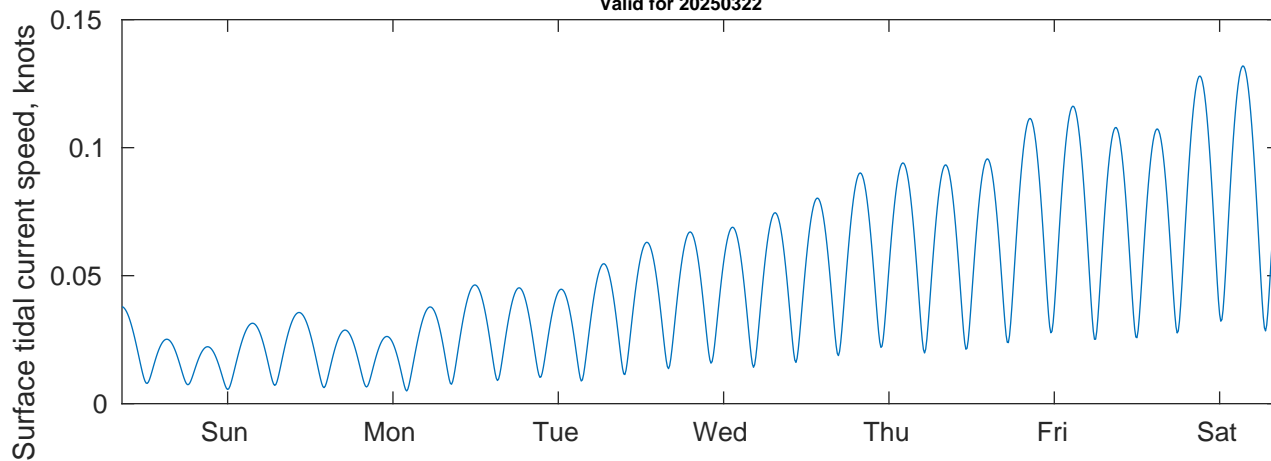
Tidal Currents and Heights for Gyre at 20250322
