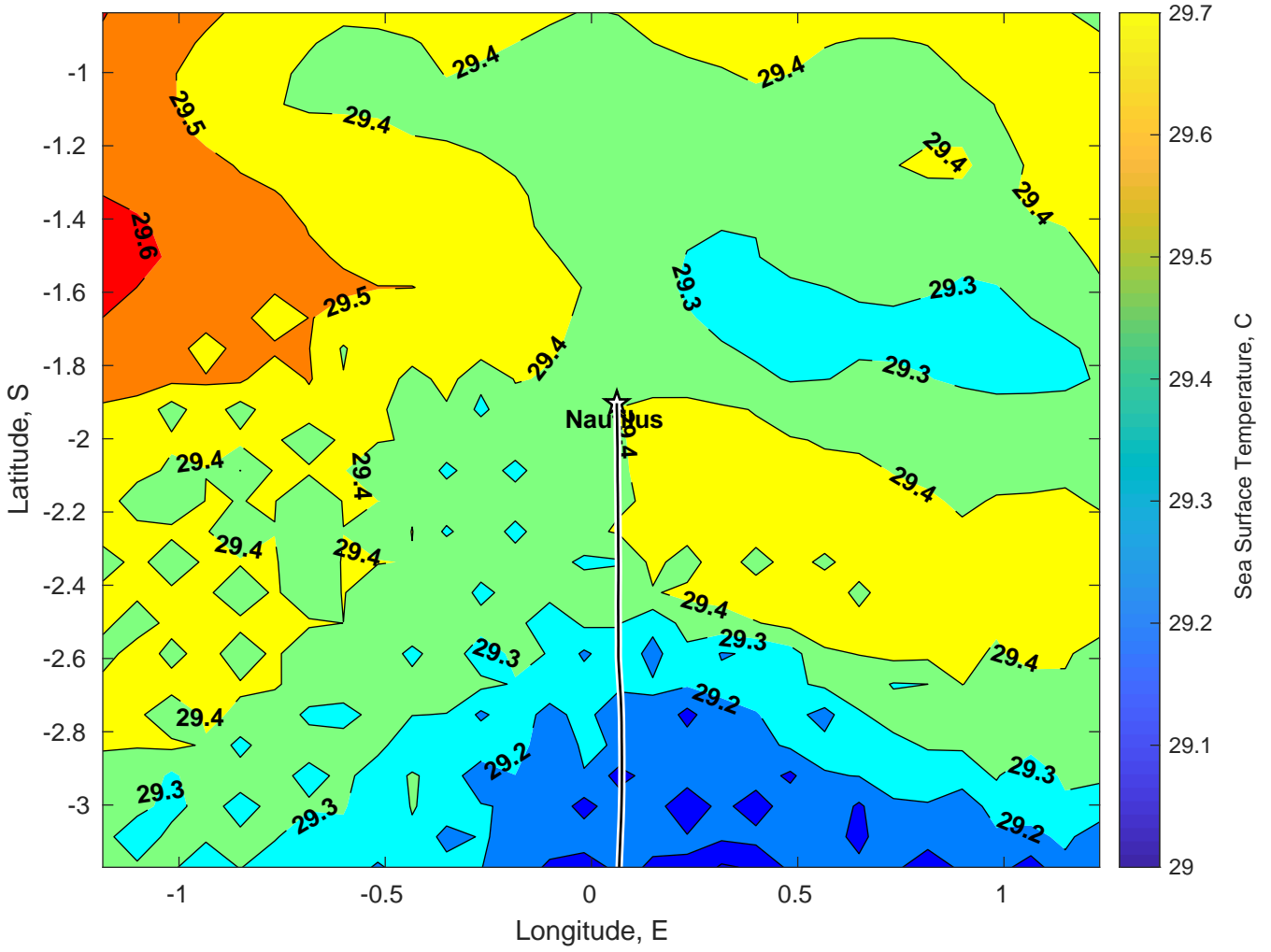
SST for Nautilus at 21-Mar-2025 00:00:00
