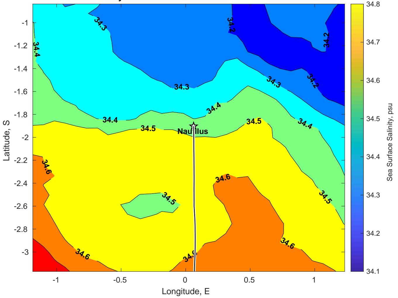
Surface Salinity for Nautilus at 21-Mar-2025 00:00:00
