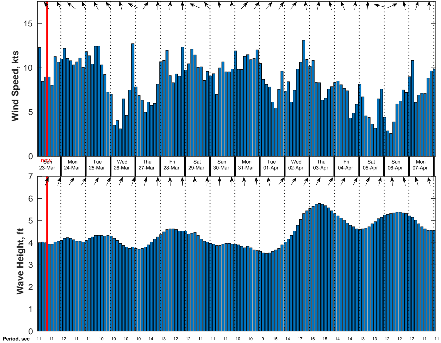
Wind & Wave Forecast for Nautilus from 22-Mar-2025 02:00:00 to 07-Apr-2025 02:00:00
