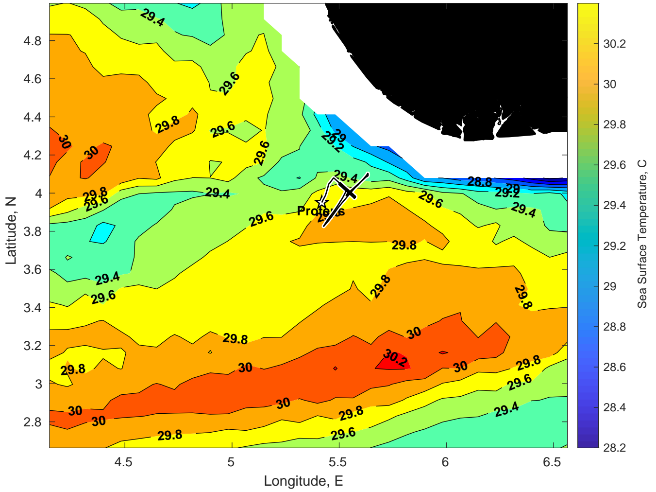
SST for Proteus at 21-Mar-2025 00:00:00
