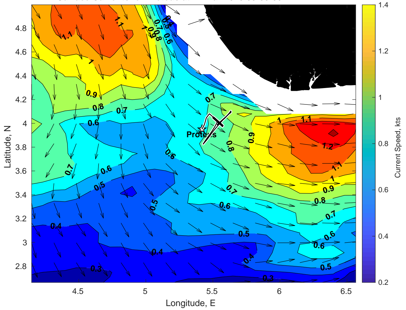
Surface Currents for Proteus at 21-Mar-2025 00:00:00
