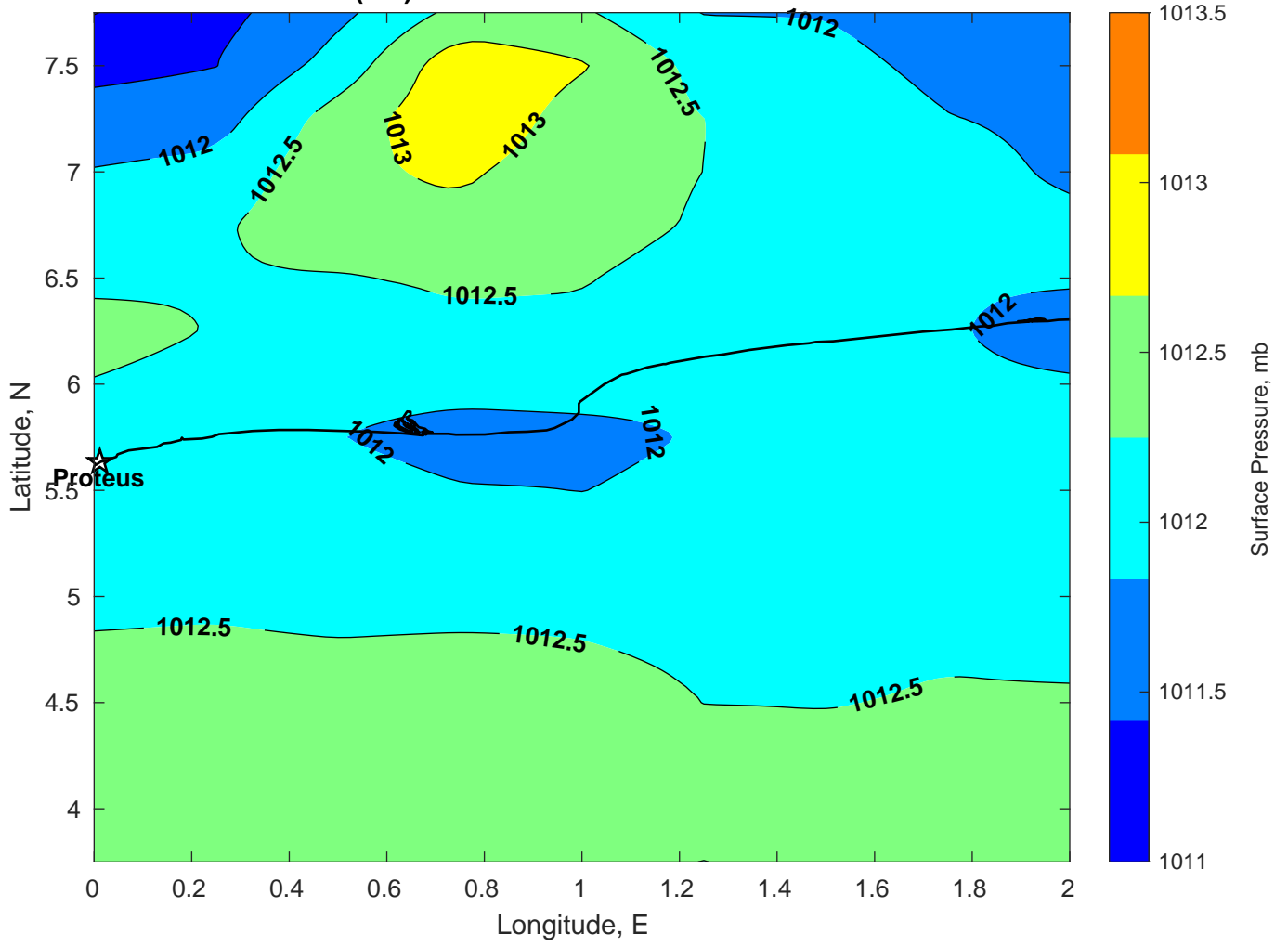
Surface Pressure (mb) for Proteus at 22-Mar-2025 00:00:00
