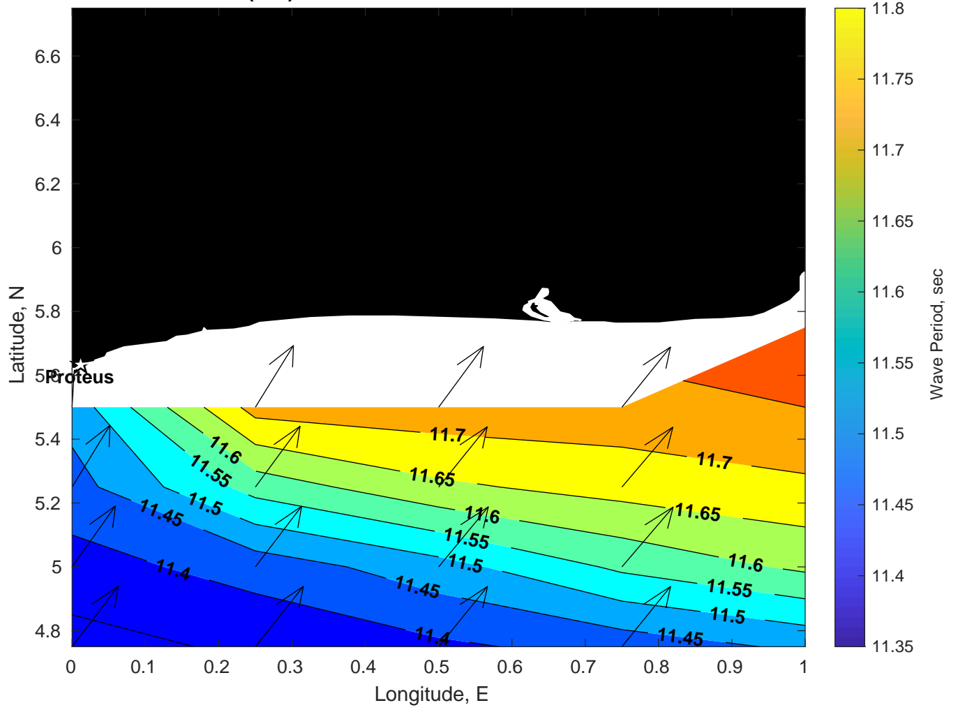
Wave Period (sec) for Proteus at 22-Mar-2025 09:00:00
