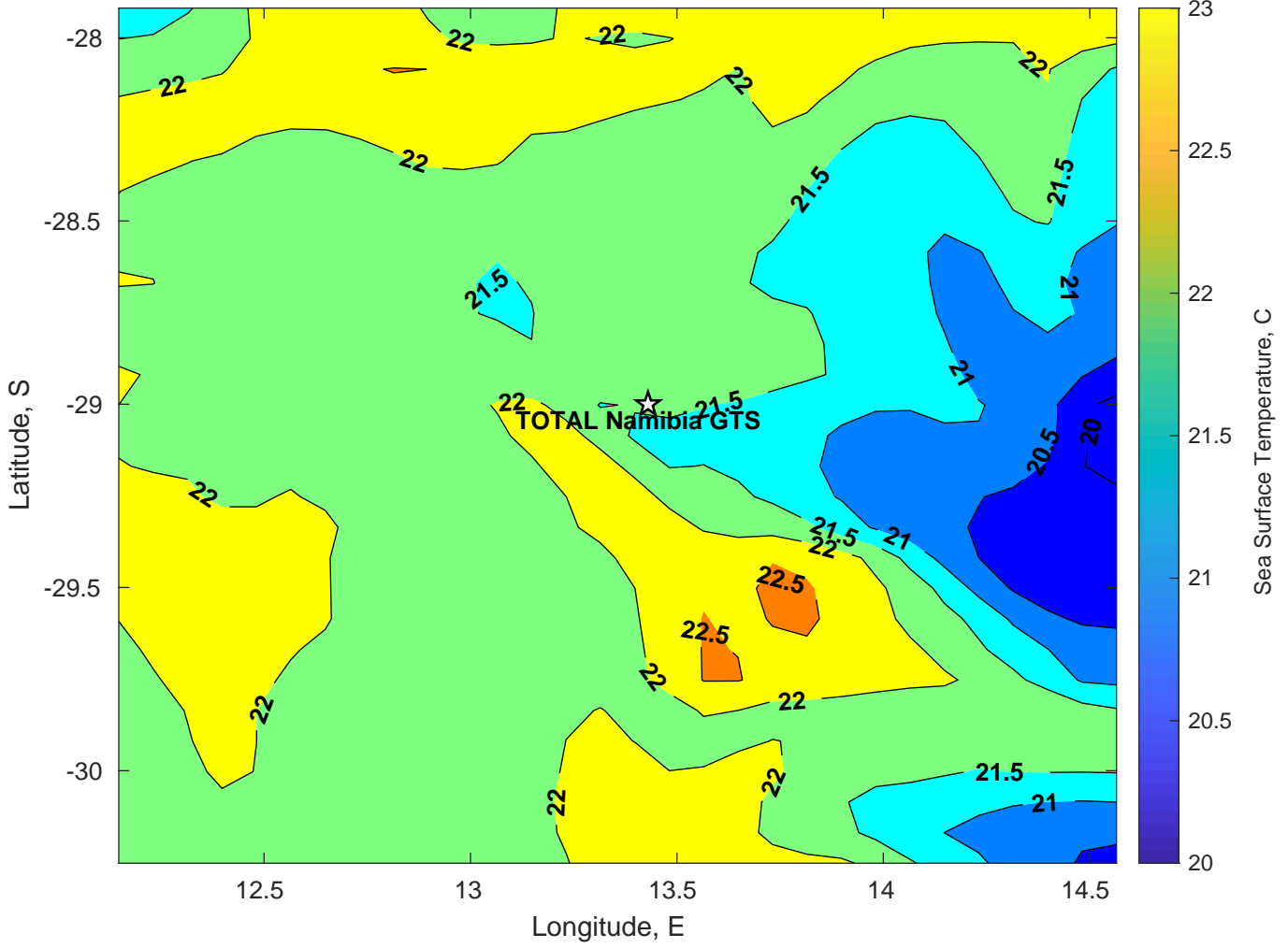
SST for TOTAL Namibia GTS at 21-Mar-2025 00:00:00
