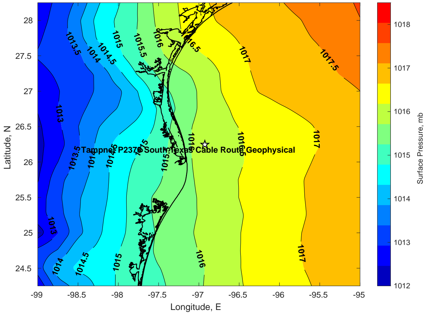
Pressure (mb) for Tampnet P2378 South Texas Cable Route Geophysical at 22-Mar-2025 00:00:00
