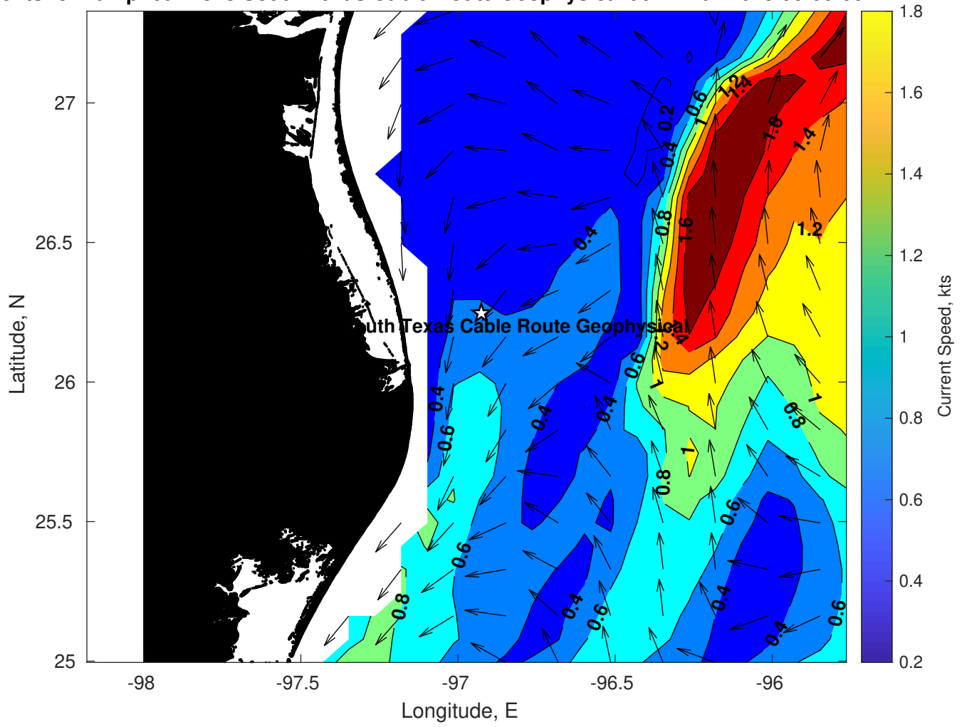
Surface Currents for Tampnet P2378 South Texas Cable Route Geophysical at 21-Mar-2025 00:00:00
