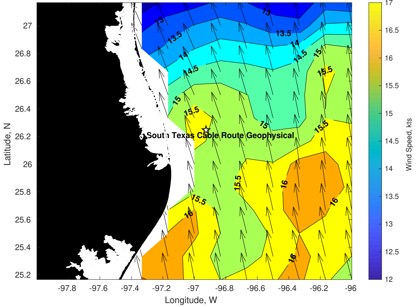
Winds (kts) for Tampnet P2378 South Texas Cable Route Geophysical at 22-Mar-2025 09:00:00
