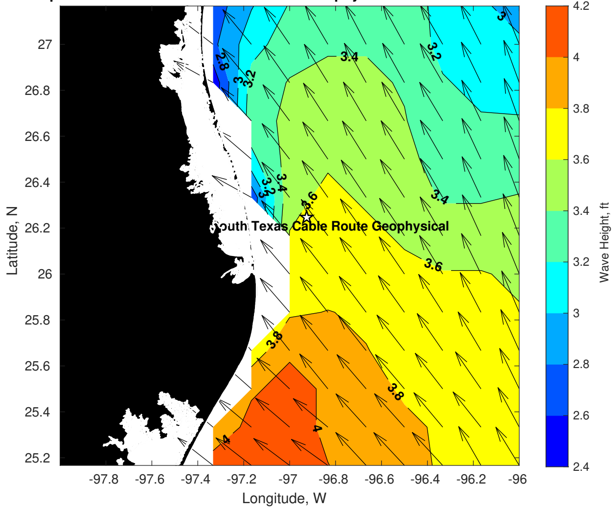
Wave Height (ft) for Tampnet P2378 South Texas Cable Route Geophysical at 22-Mar-2025 09:00:00
