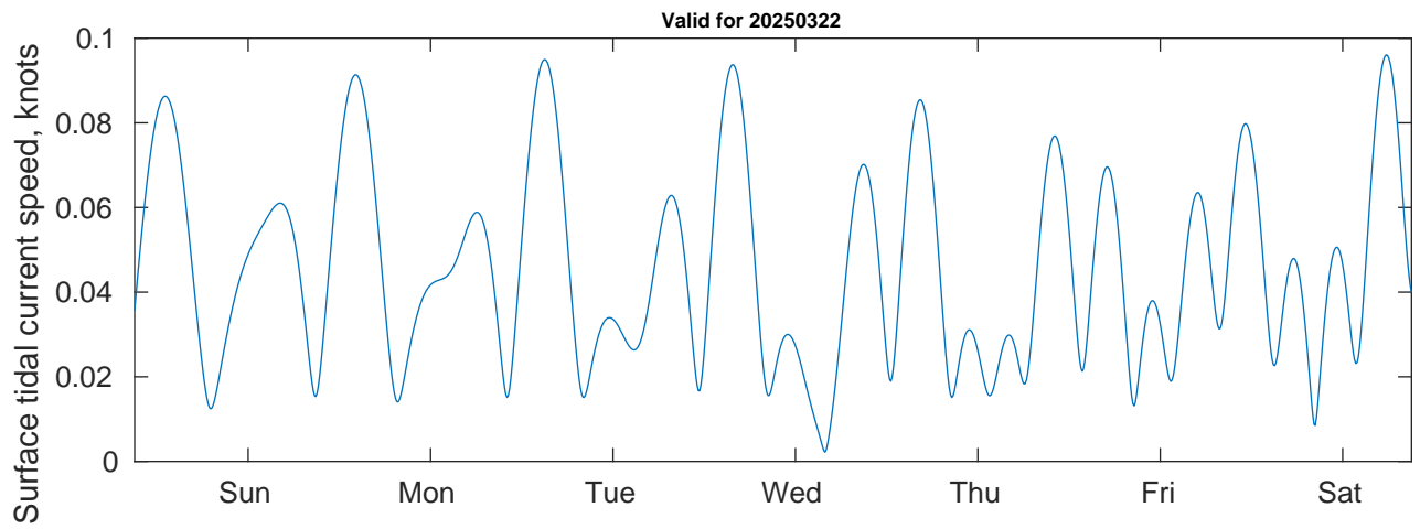
Tidal Currents and Heights for Tampnet P2378 South Texas Cable Route Geophysical at 20250322
