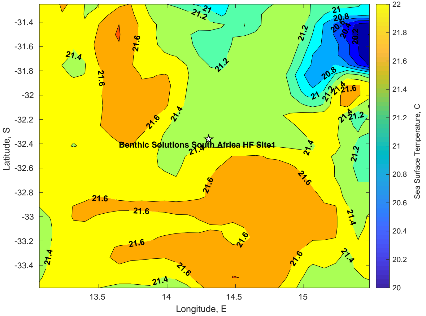
SST for Benthic Solutions South Africa HF Site1 at 22-Mar-2025 00:00:00
