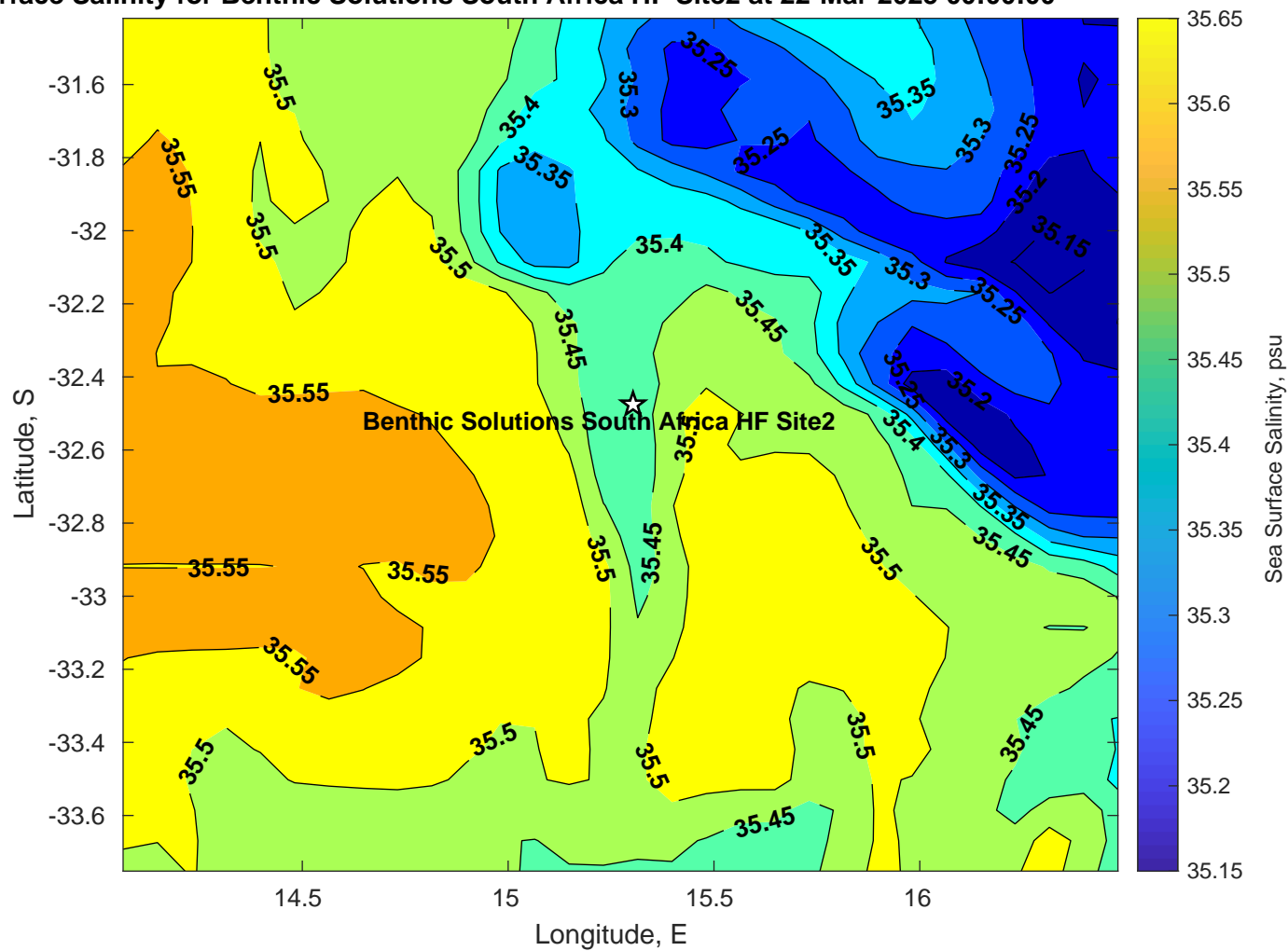
Surface Salinity for Benthic Solutions South Africa HF Site2 at 22-Mar-2025 00:00:00
