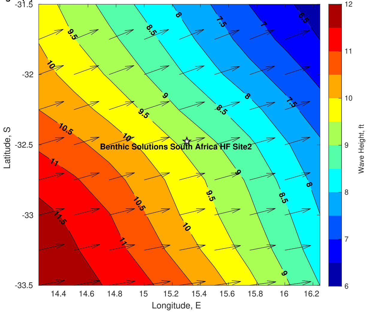
Wave Height (ft) for Benthic Solutions South Africa HF Site2 at 23-Mar-2025 09:00:00
