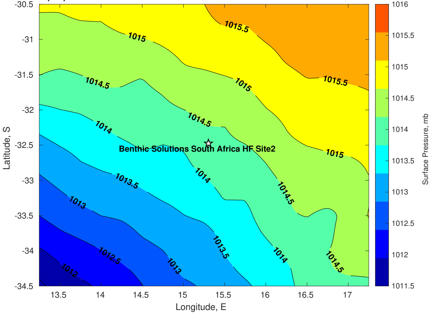
Surface Pressure (mb) for Benthic Solutions South Africa HF Site2 at 24-Mar-2025 00:00:00
