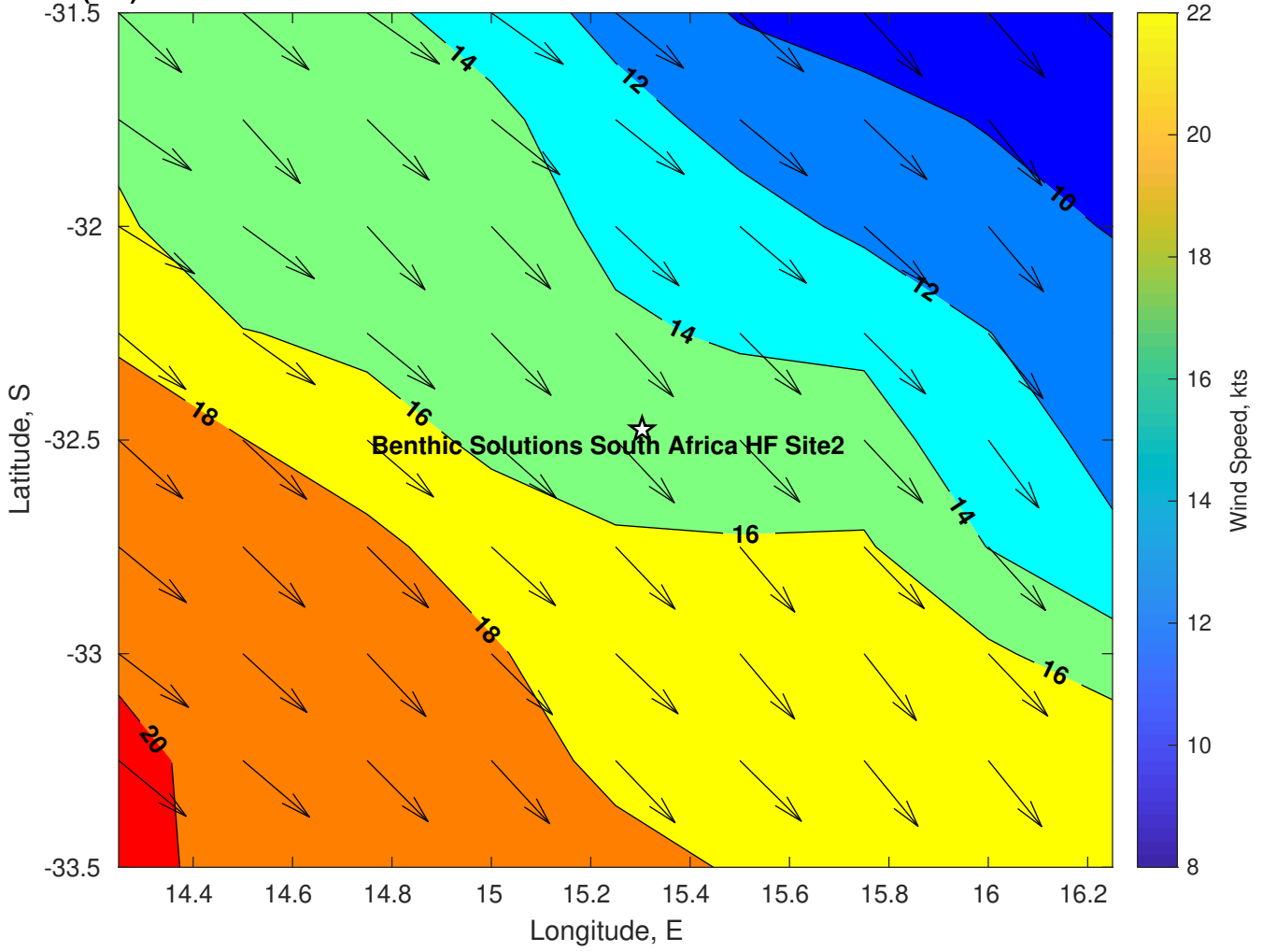
Winds (kts) for Benthic Solutions South Africa HF Site2 at 23-Mar-2025 09:00:00
