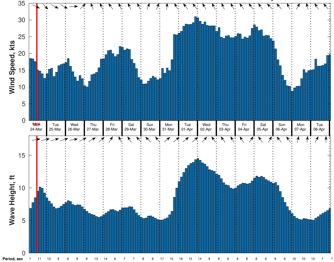
Wind & Wave Forecast for Benthic Solutions South Africa HF Site2 from 23-Mar-2025 02:00:00 to 08-Apr-2025 02:00:00
