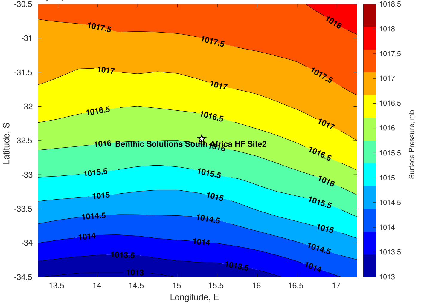
Surface Pressure (mb) for Benthic Solutions South Africa HF Site2 at 25-Mar-2025 00:00:00
