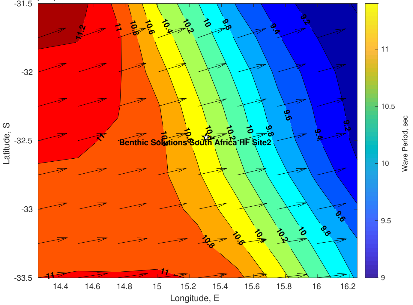
Wave Period (sec) for Benthic Solutions South Africa HF Site2 at 23-Mar-2025 09:00:00
