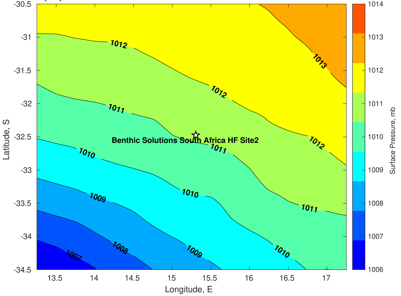
Surface Pressure (mb) for Benthic Solutions South Africa HF Site2 at 23-Mar-2025 00:00:00
