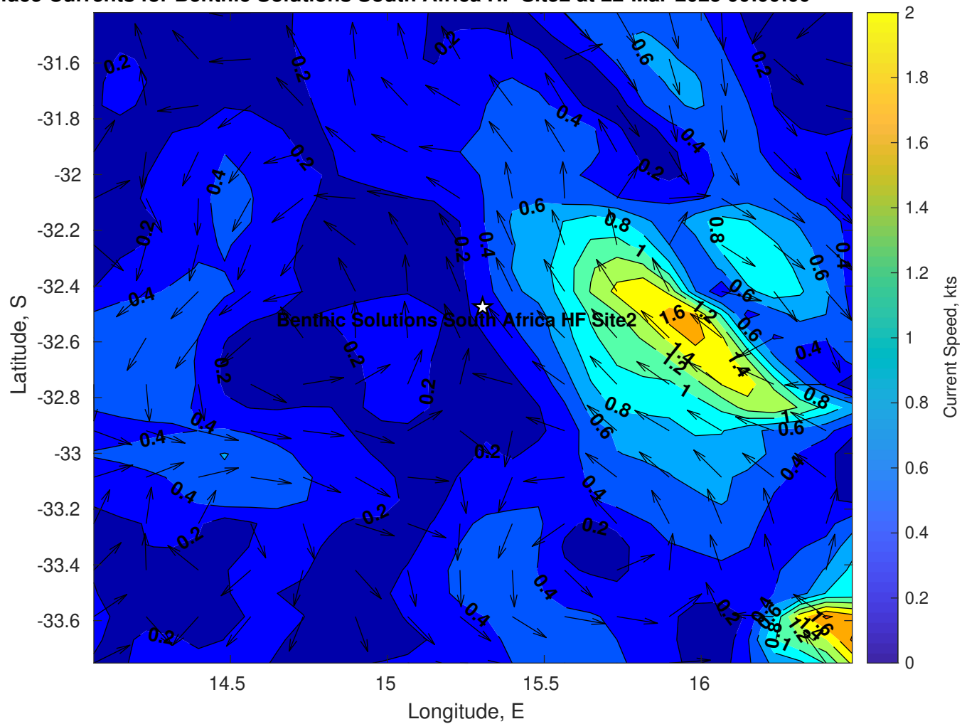
Surface Currents for Benthic Solutions South Africa HF Site2 at 22-Mar-2025 00:00:00
