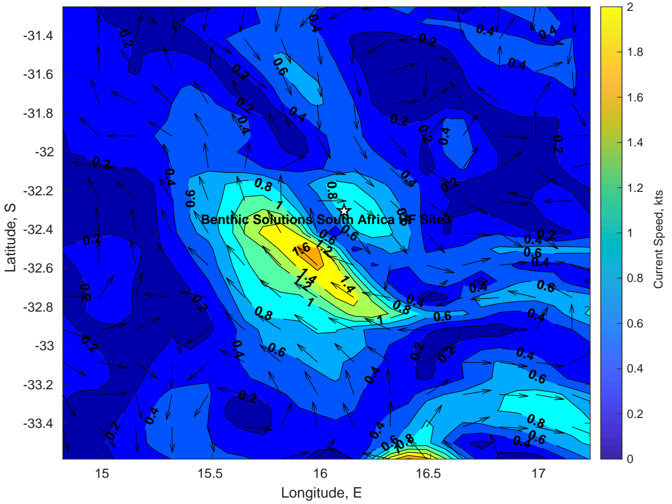
Surface Currents for Benthic Solutions South Africa HF Site3 at 22-Mar-2025 00:00:00
