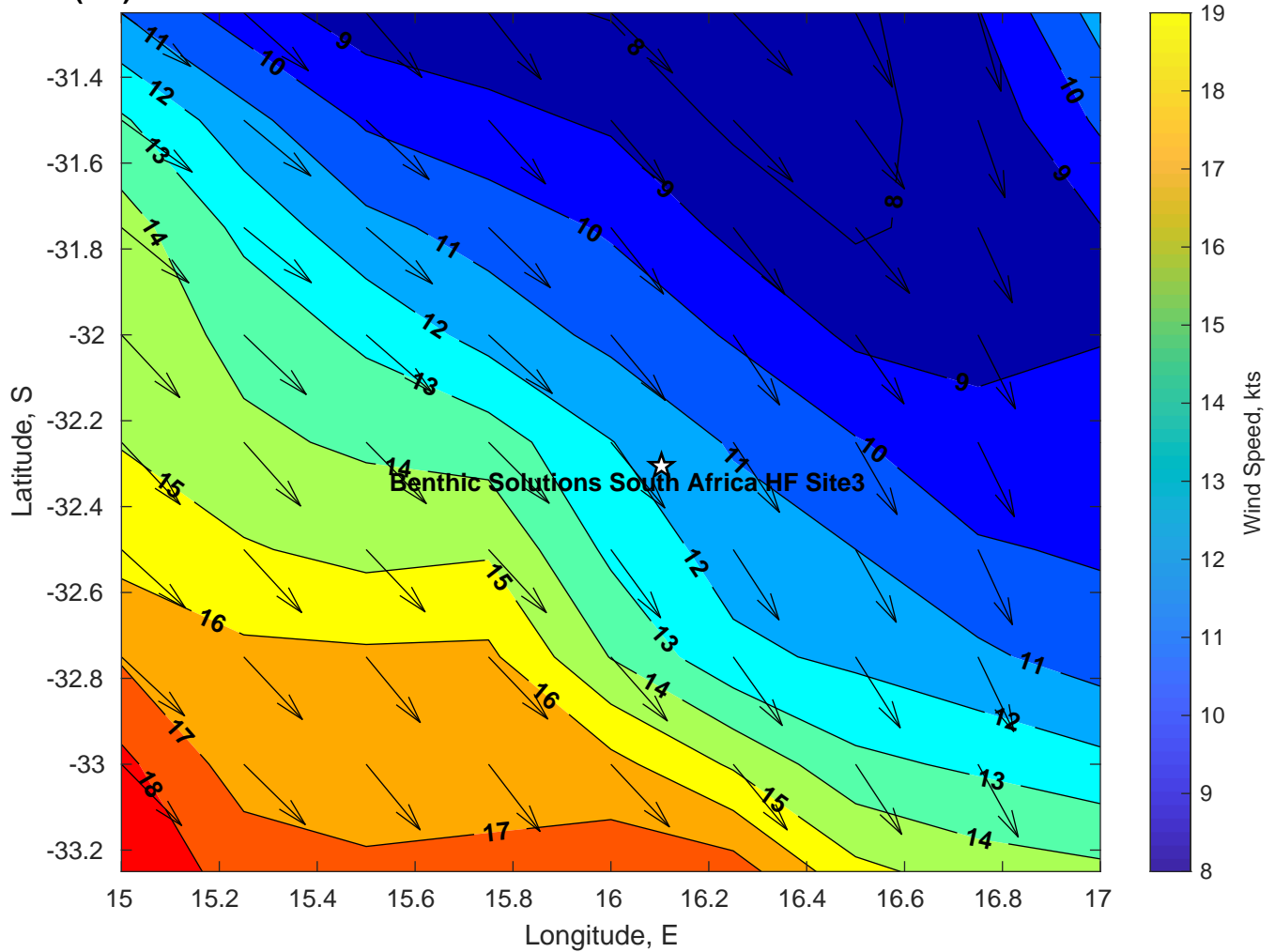
Winds (kts) for Benthic Solutions South Africa HF Site3 at 23-Mar-2025 09:00:00
