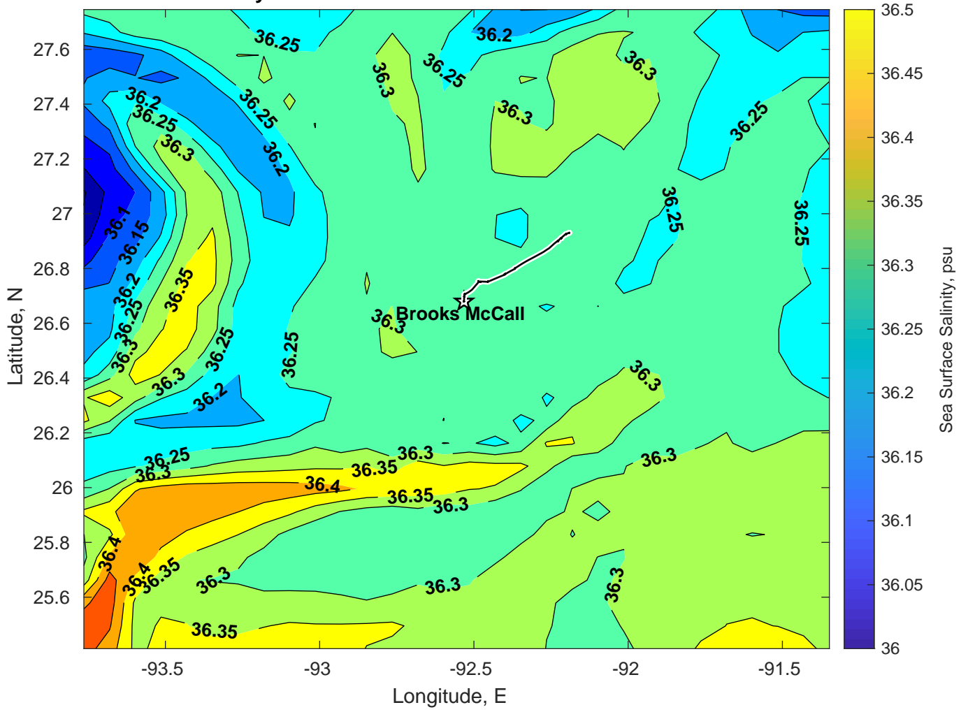
Surface Salinity for Brooks McCall at 22-Mar-2025 00:00:00
