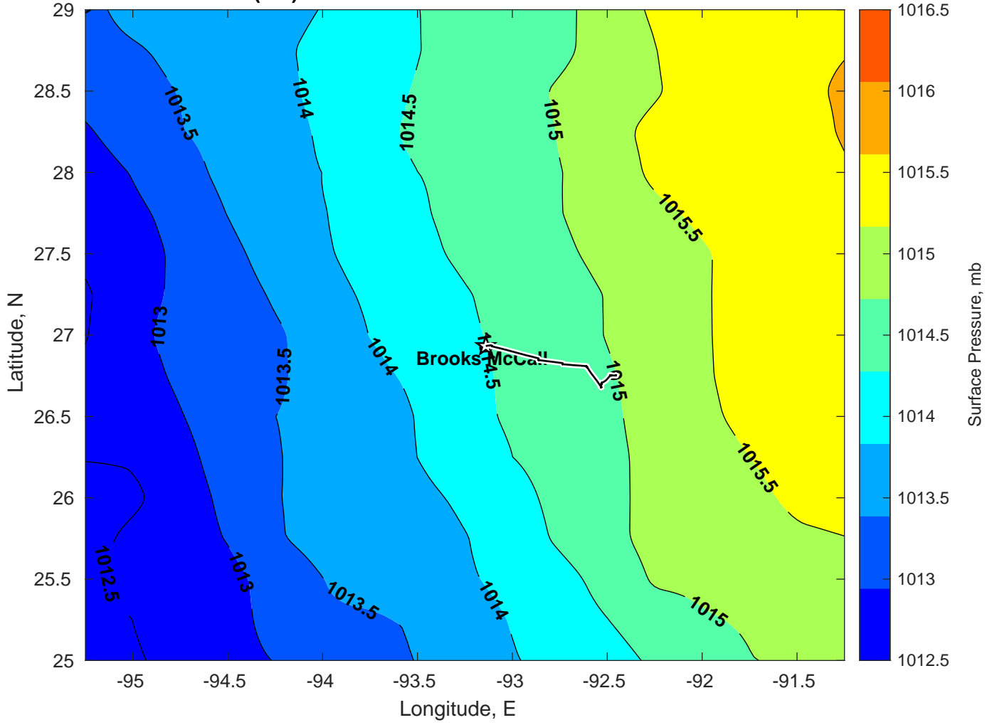
Surface Pressure (mb) for Brooks McCall at 24-Mar-2025 00:00:00
