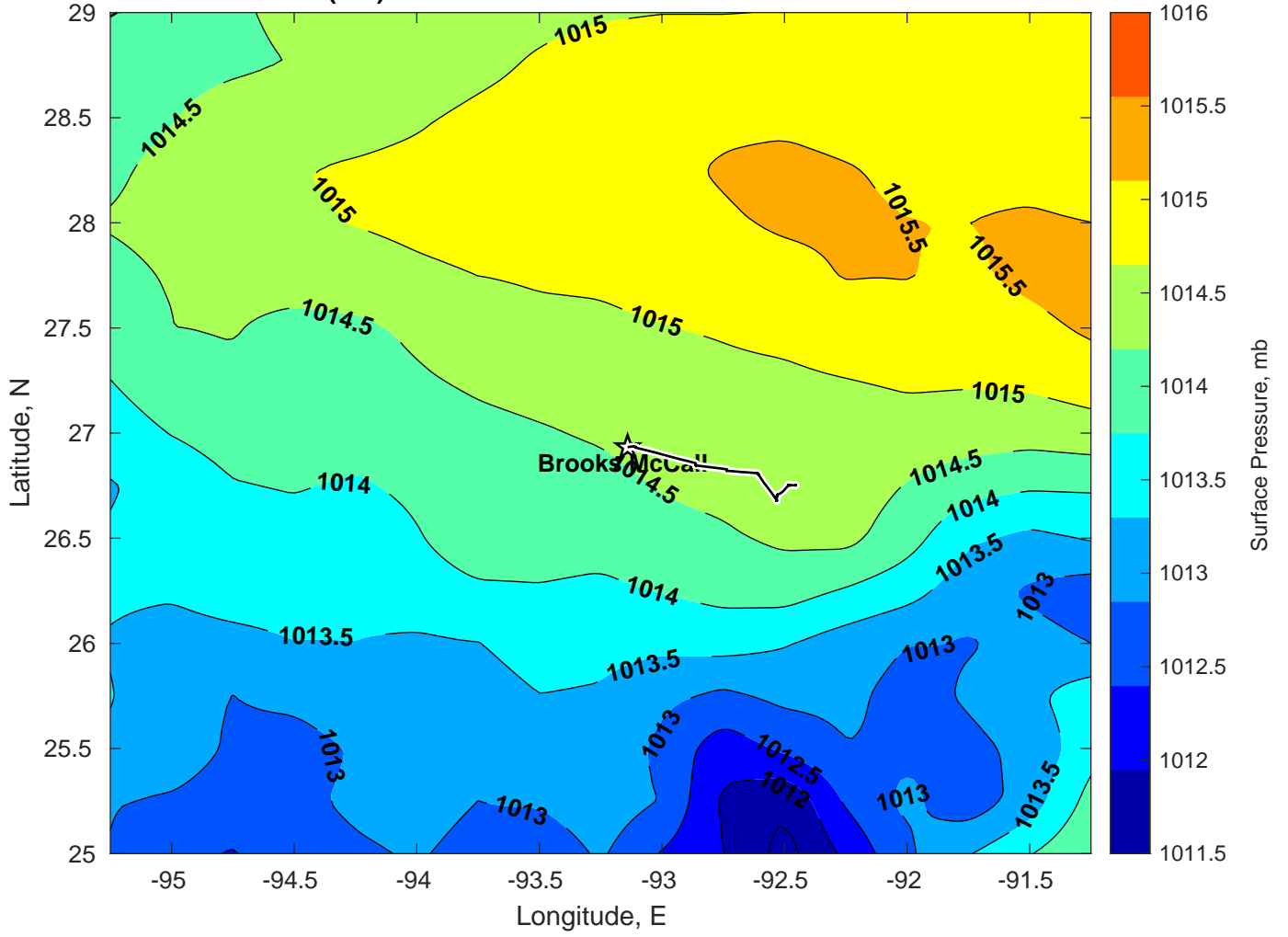
Surface Pressure (mb) for Brooks McCall at 25-Mar-2025 00:00:00
