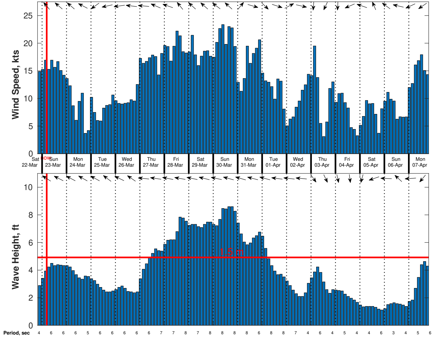
Wind & Wave Forecast for Brooks McCall from 22-Mar-2025 20:00:00 to 07-Apr-2025 20:00:00
