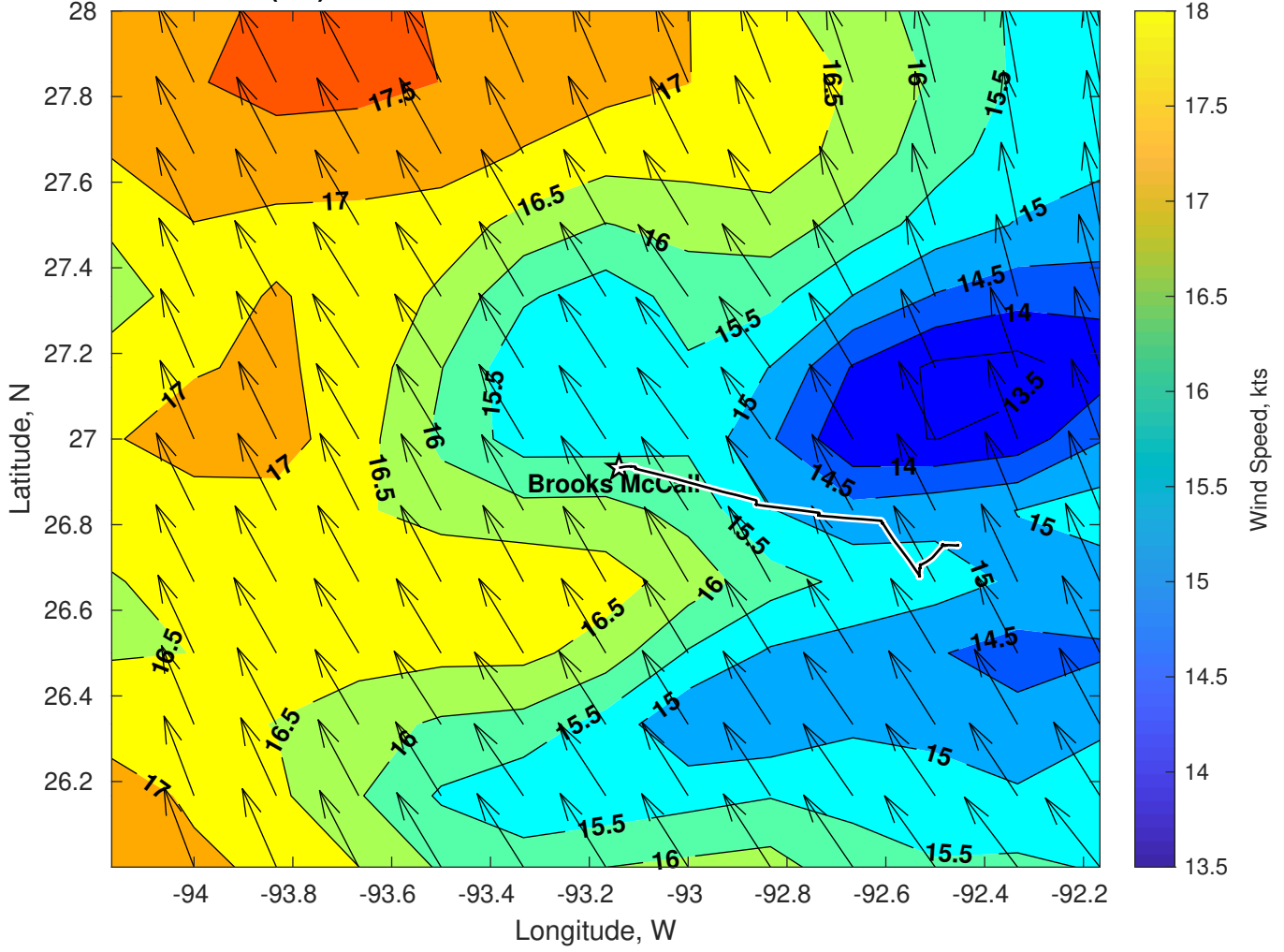
Winds (kts) for Brooks McCall at 23-Mar-2025 09:00:00
