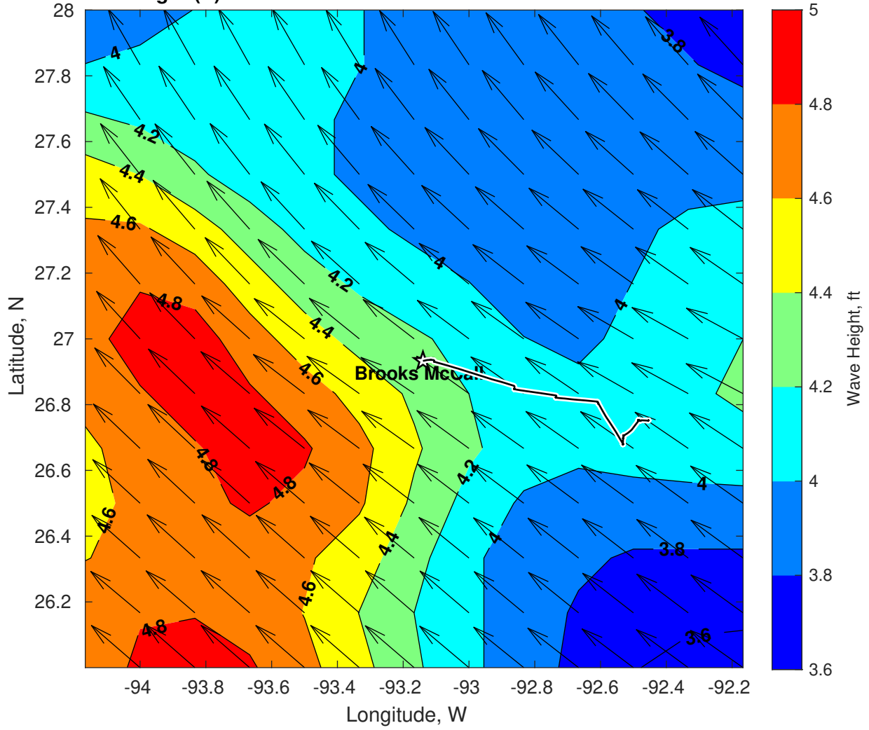
Wave Height (ft) for Brooks McCall at 23-Mar-2025 09:00:00
