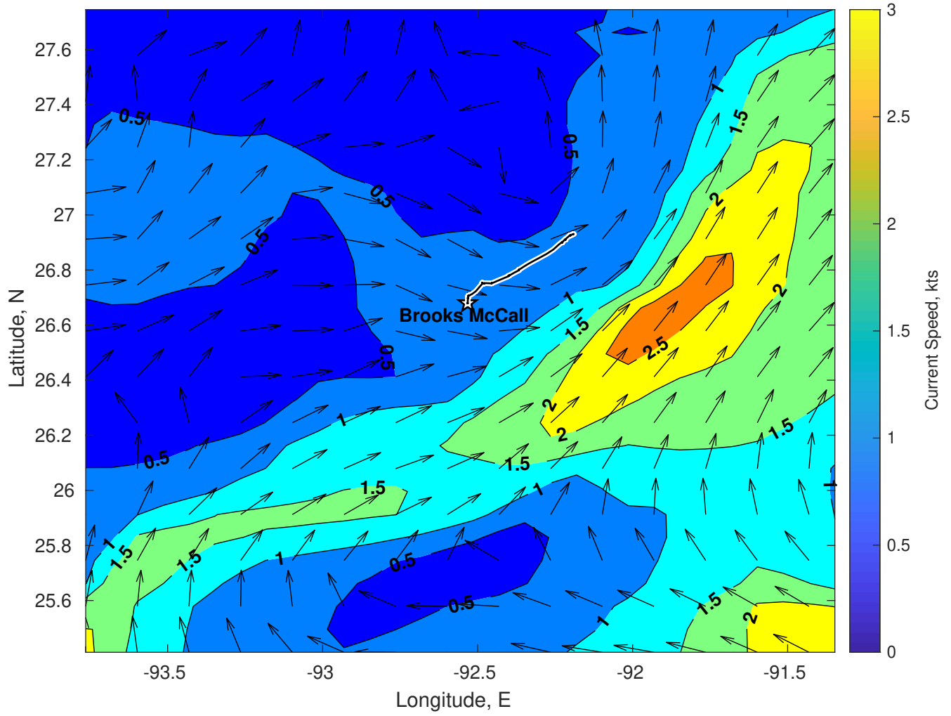
Surface Currents for Brooks McCall at 22-Mar-2025 00:00:00
