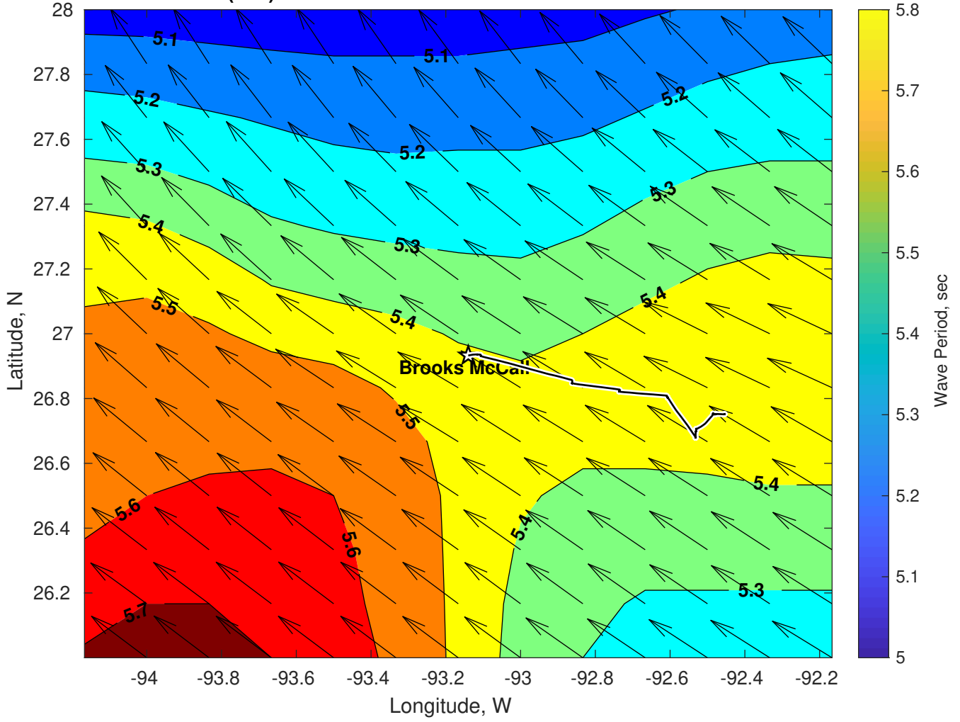
Wave Period (sec) for Brooks McCall at 23-Mar-2025 09:00:00
