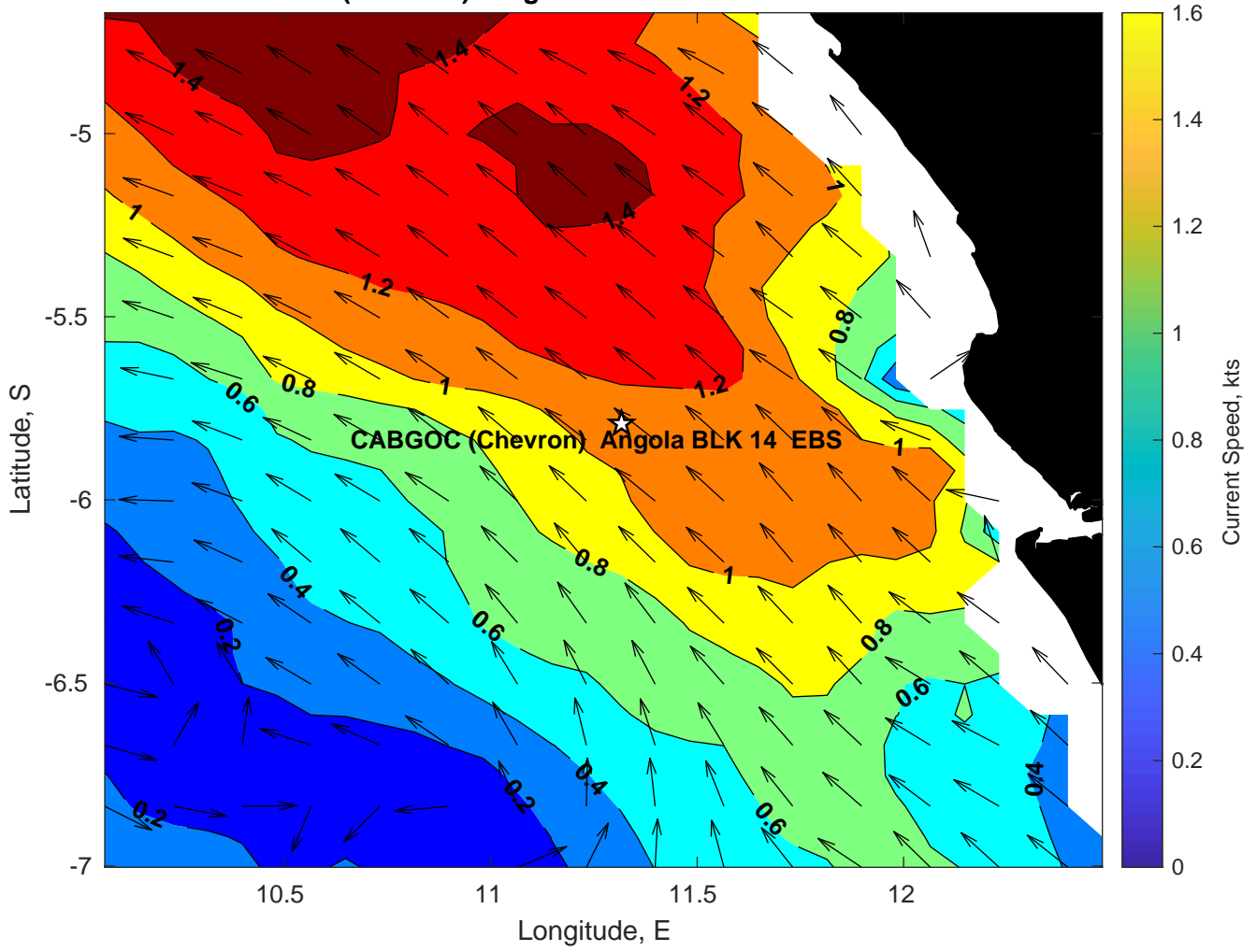
Surface Currents for CABGOC (Chevron) Angola BLK 14 EBS at 22-Mar-2025 00:00:00
