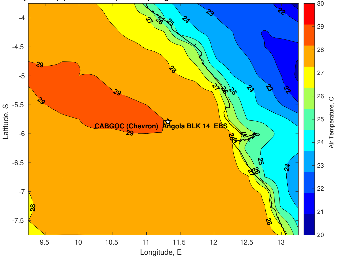
Air Temperature (C) for CABGOC (Chevron) Angola BLK 14 EBS at 23-Mar-2025
