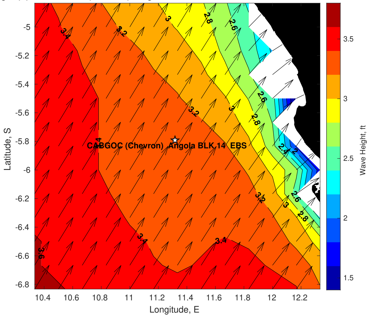
Wave Height (ft) for CABGOC (Chevron) Angola BLK 14 EBS at 23-Mar-2025 09:00:00
