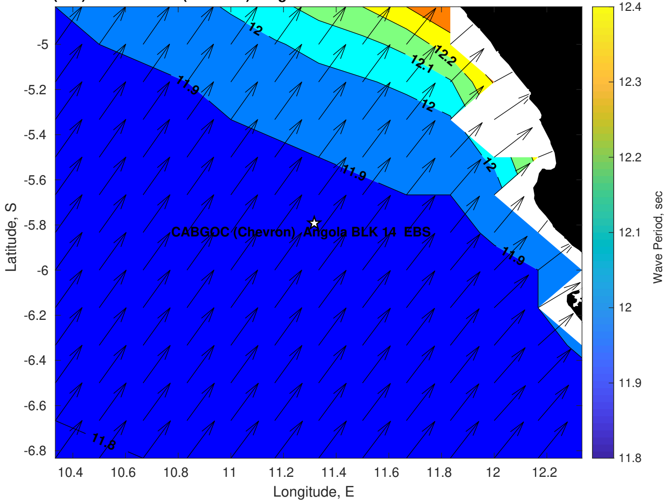
Wave Period (sec) for CABGOC (Chevron) Angola BLK 14 EBS at 23-Mar-2025 09:00:00
