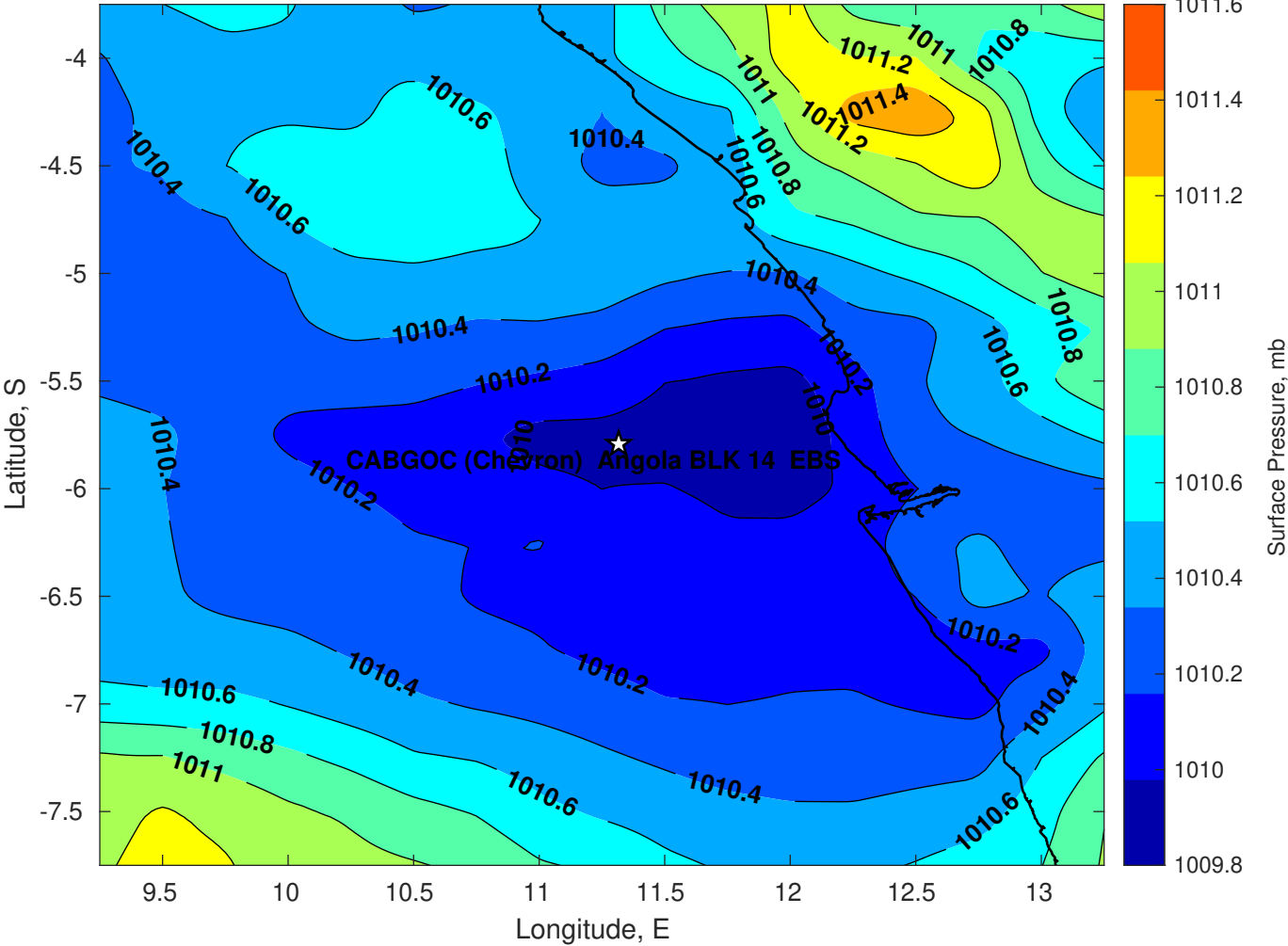
Surface Pressure (mb) for CABGOC (Chevron) Angola BLK 14 EBS at 25-Mar-2025 00:00:00
