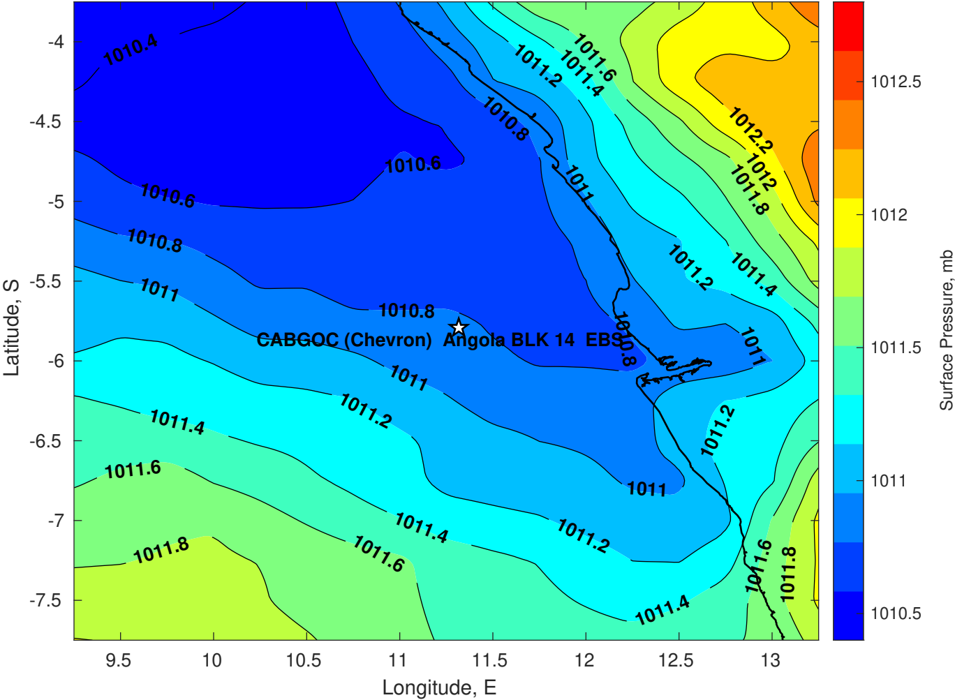
Surface Pressure (mb) for CABGOC (Chevron) Angola BLK 14 EBS at 23-Mar-2025 00:00:00
