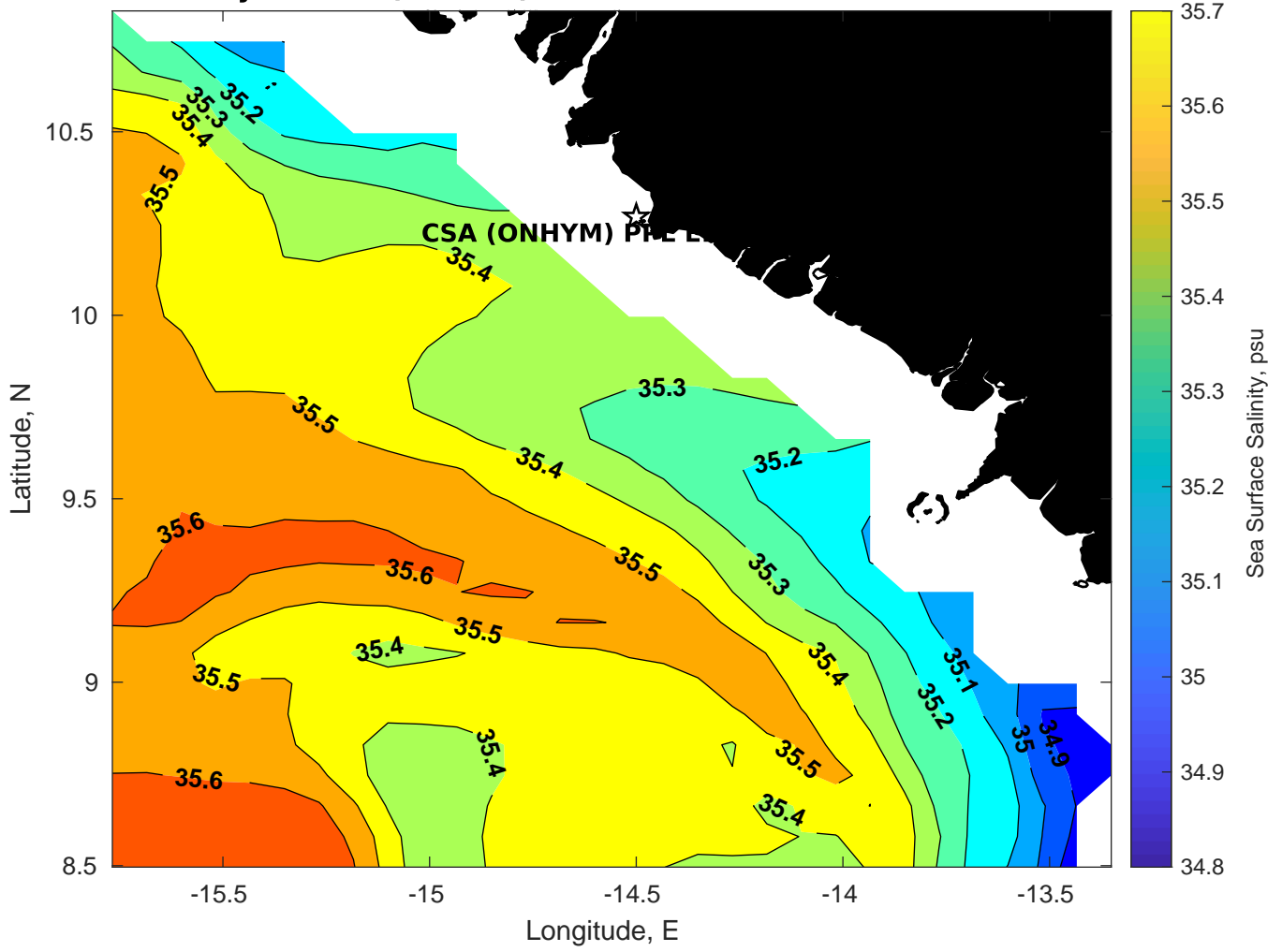
Surface Salinity for CSA (ONHYM) PPL EBS - Guinea at 22-Mar-2025 00:00:00
