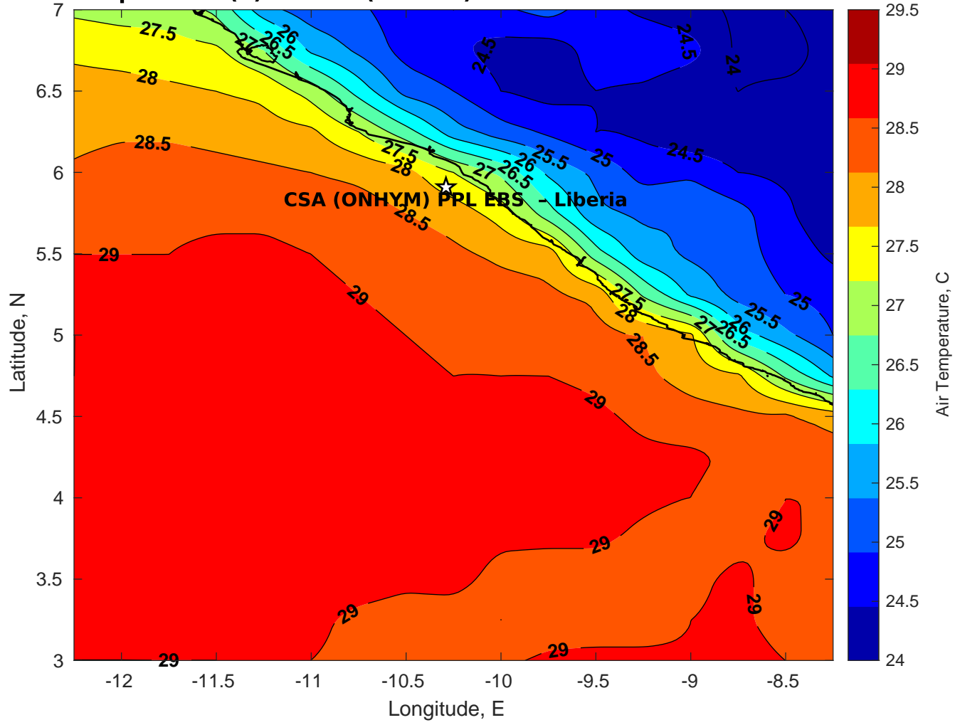
Air Temperature (C) for CSA (ONHYM) PPL EBS - Liberia at 23-Mar-2025
